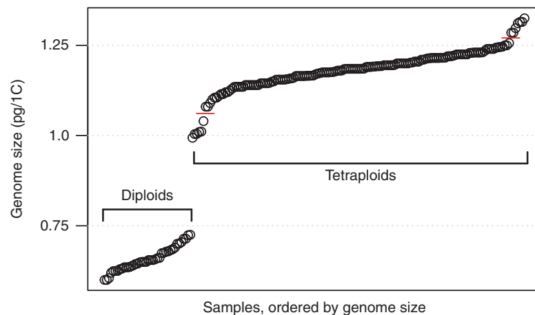
FIG. 3. Patterns of genome size variation in British Euphrasia . (A) The distribution of population-average genome size for 90 populations of 23 taxa (13 species and ten hybrids). Vertical bars indicate the genome size range within each population where more than one individual was analysed. (B) Distribution of individual genome size estimates for all 192 samples. Horizontal red lines indicate the limits of the continuous part of the tetraploid genome size distribution. (C) Population-average genome sizes plotted against latitude for the three most widely sampled species. The solid purple line indicates a significant statistical relationship of genome size with latitude across 17 populations of E. arctica . This relationship was only marginally significant for 11 populations of E. anglica (dashed blue line). No significant association was found across nine populations of the highly selfing E. micrantha .
