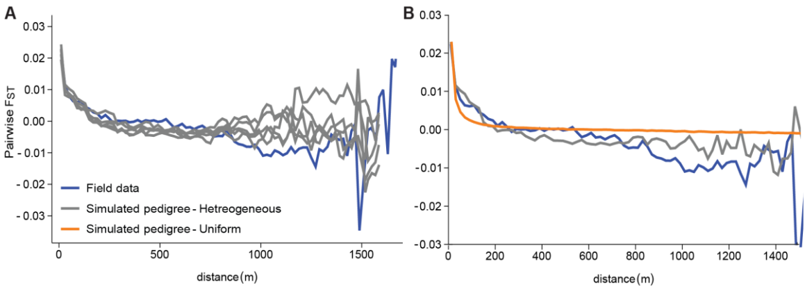
Figure 4. A: Isolation by distance compared between the field data (blue) and five replicate simulated pedigrees (gray) based on a heterogeneous population density. B: Isolation by distance from the field data (blue) compared between the simulated pedigree with a heterogeneous (gray) and uniform (orange) population density.
