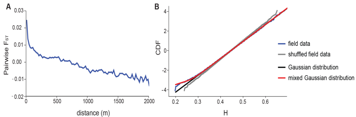
Figure 2. A: Pairwise relatedness ( F_{ST} ) between individuals decreases rapidly with geographic distance showing isolation-by-distance in the field data. B: Probit transform of the cumulative distribution function (CDF) of the distribution of individual heterozygosity (H). A Gaussian appears as a straight line on a probit scale, and the y-axis is the number of standard deviations of the standard normal distribution.
