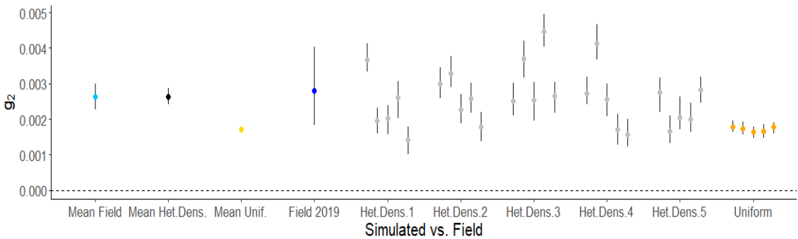
Figure 5. Identity disequilibrium ( g_2 ) calculated from field data versus simulated pedigrees. Five of ten replicates per pedigree are shown (gray: heterogeneous density, with five simulated pedigrees; orange: uniform density, with one simulated pedigree). Mean from the field (light blue) is across 2009-2019, while mean from the heterogeneous (black) and uniform (yellow) simulations is across all replicates. The final year of field data (dark blue) is comparable to g_2 calculated from the final year of pedigree replicates (gray and orange).
