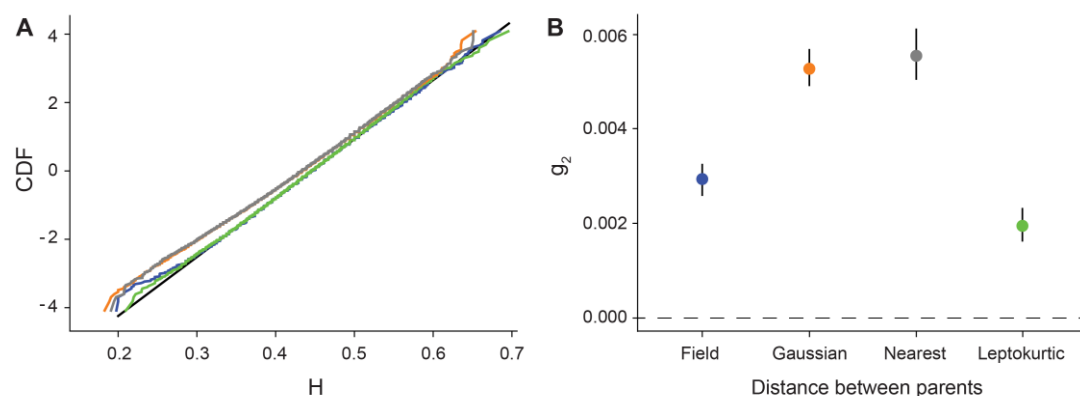
Figure 3. A: Probit transform of the CDF of multilocus heterozygosity, H , for the field data (blue) versus a single replicate of offspring simulated from Gaussian pollen dispersal (orange), nearest neighbor matings (gray), and leptokurtic pollen dispersal (green). A normal distribution (black) with the same mean and standard deviation as the field data is included for comparison B: Identity disequilibrium for the same data as above indicating mean and 95% CI.
