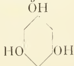
Phloroglucine
