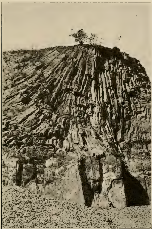
First Watchung Mountain: quarry West Orange— showing columnar structure.
