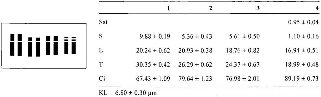
Fig. 5: Karyotype of Crepis pannonica subsp. pannonica with relevant chromosome parameters. Abb. 5: Idiogramm und relevante Chromosomen-Parameter von Crepis pannonica subsp. pannonica .
