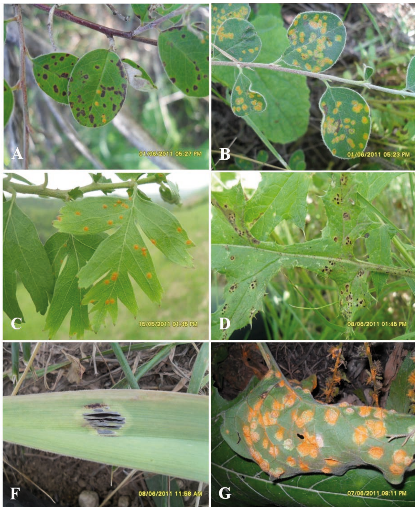
Fig. 3: Gymnosporangium fusiforme on Cotoneaster pseudomultiflorus (rust: A . on the upper leaf surface with other fungal spot, B . on the lower surface); Gymnosporangium confusum on Crataegus pseudoheterophylla subsp. turkestanica ( C . on the upper and lower leaf surface); Puccinia calycitrapae on Cirsium sp. ( D . On the upper surface of host leaves); Puccinia eremuri on Eremurus regelii ( E . on the upper leaf surface with dark brown color); Puccinia eremuri on Eremurus regelii ( F . on the upper leaf surface with dark brown color); Puccinia cousiniae on Cousinia umbrosa ( G . on the lower leaf surface). Photographs by Yusufjon Gafforov.
