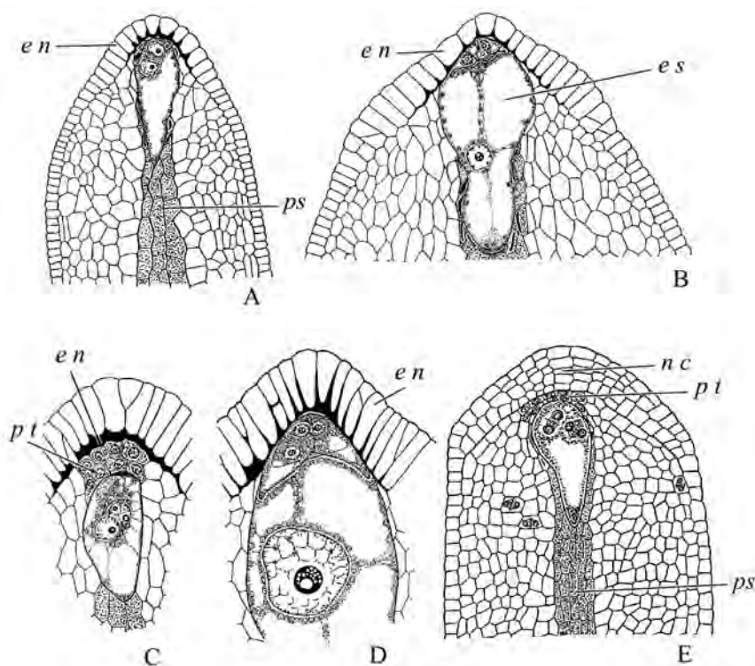
Figure 11. Transformations of the nucellus epidermis in representatives of Nymphaeaceae. A – Nymphaea alba , B – N. gigantea , C, D – Victoria cruciana , E – Nuphar lutea . en – epidermis of nucellus, es – embryo sac, nc – nucellar cap, ps – postament, pt – parietal tissue.
