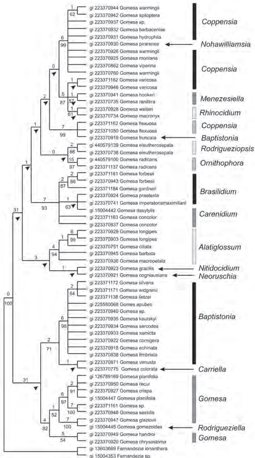
Figure 7. One of the most parsimonious trees for Gomesa s.l. species of marK gene. Length of branches is shown above; values below branches represent bootstrap support (≥ 50%); arrows indicate clades that collapse in the strict consensus tree; gi denotes the ID number of GenBank.
