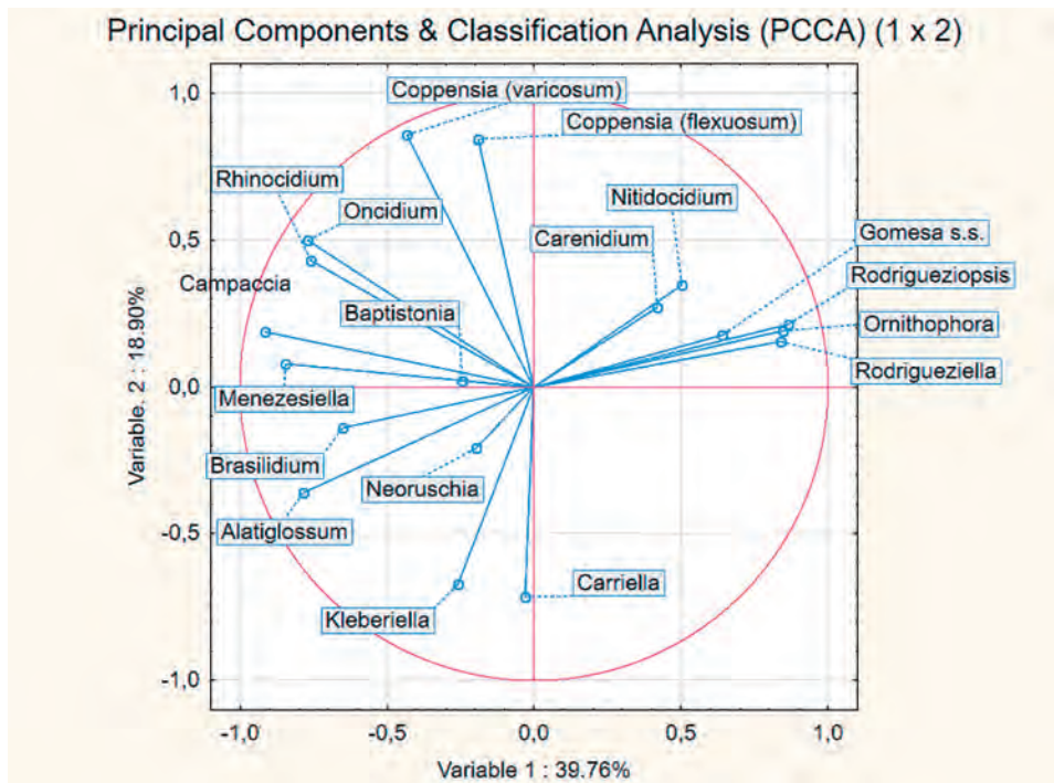
Figure 3. Morphological variation in Gomesa s.l. Principal components and classification analysis (PCCA) using all variables for analysis.
