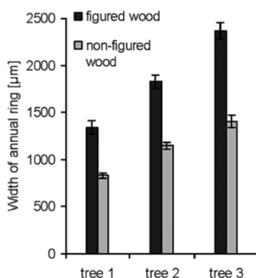
Figure 4. Average width of annual ring in Karelian birch trees in zones with figured and non-figured wood within a single cross-section.
