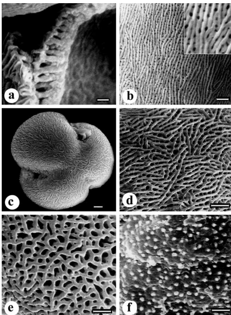
Figure 2: SEM micrographs of pollen grains in Veronica : a) cross section of the exine of V. capillipes ; b) rugulate-Perforate tectum of V. acrotheca ; c) pollen of V. gentianoides at polar view; d) rugulate-Perforate tectum of V. gentianoides ; e) microreticulate tectum of V. beccabunga ; f) scabrate tectum of V. hederifolia . a, b) scale bar = 500 nm; c) scale bar = 2 \mu m; d–f) scale bar = 1 \mu m.
