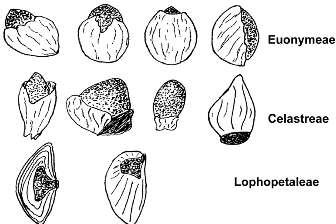
Figure 4: Morphological diversity of seeds in the tribes Euonymaceae, Celastreae and Lophopetaleae.
