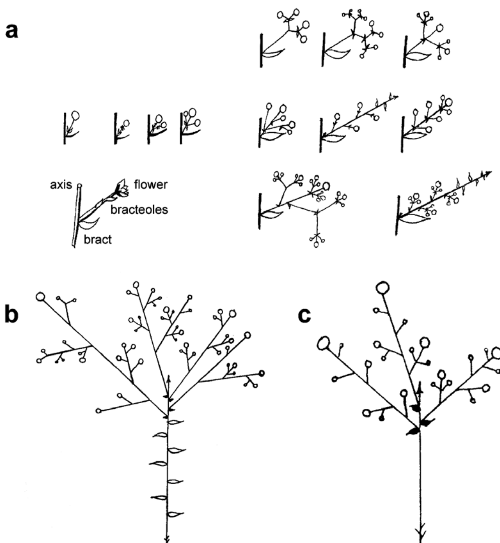
Figure 1: Structure of inflorescences in representatives of the Celastreae tribe: a: axillary floral position in different genera; b–c: pseudoterminal inflorescences in Bhesa paniculata Wall. (b) and B. ceylanica Arn. (c).
