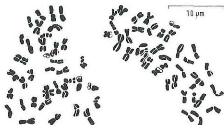
Fig. 12. Onosma malkarmayorum , two mitotic metaphase plates from root tips, with 2n = 38 chromosomes, material from Beden. Cult. no BOR 1206.
