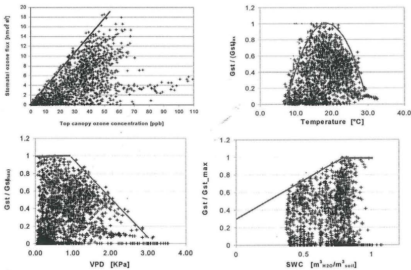
Fig. 2. Border-line analysis for the stomatal conductance (upper left frame) and the ratio Gst/Gst_{max} (other frames) as functions of ozone concentration, temperature, vapour pressure deficit, and soil water content.
