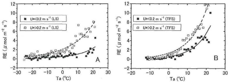
Fig. 2. Ecosystem respiration (RE) as a function of the air temperature ( T_a ) at LS (A) and TFS (B) on calm (■ and solid line: U^* < 0.20 \text{ m s}^{-1} ) and windy (□ and dash line: U^* \geq 0.20 \text{ m s}^{-1} ) nights. The curves are empirical regression results with RE = 0.401e^{0.0862T_a} ( U^* < 0.20 ) and RE = 2.0221e^{0.0649T_a} ( U^* \geq 0.20 ) for LS and RE = 0.5448e^{0.116T_a} ( U^* < 0.20 ) and RE = 1.301e^{0.1048T_a} ( U^* \geq 0.20 ) for TFS.
