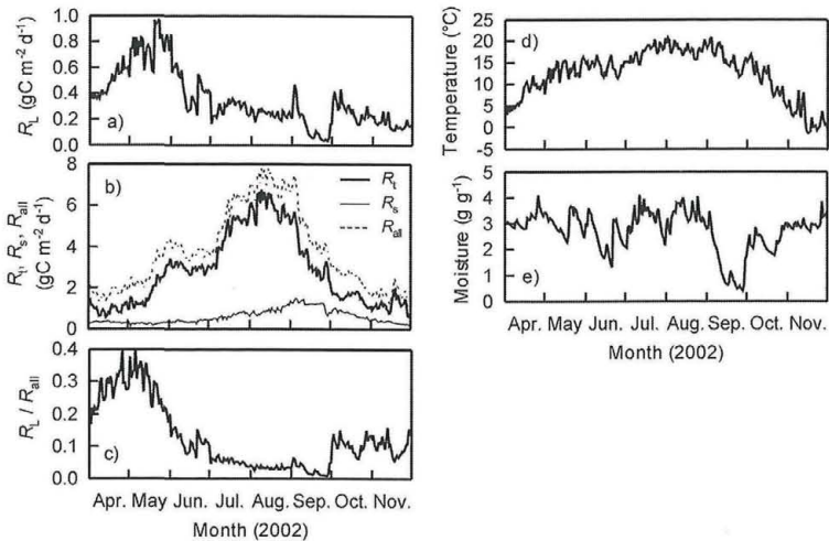
Fig. 1. Seasonal variations in daily means of R_L , R_s , R_t , R_L / R_{all} , litter temperature and litter moisture from 1 April to 30 December 2002 for the broadleaf forest.
