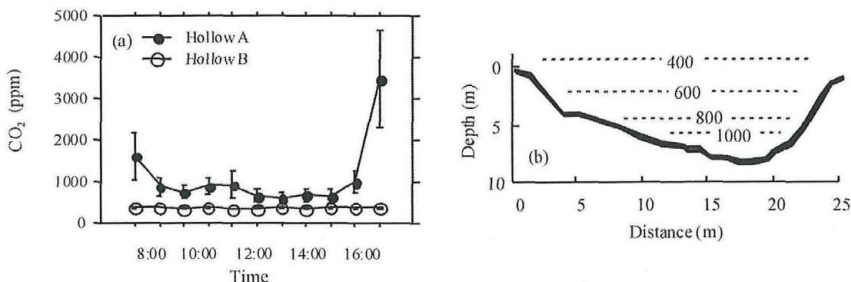
Fig. 1. (a) CO 2 concentration at 1 m height above the soil surface at the bottom of Hollow A and B for six days in July and September. Means with 95% confidence limits are shown. (b) Topography of Hollow A (thick line) with distribution of mean daytime concentration of CO 2 (μmol mol -1 ).
