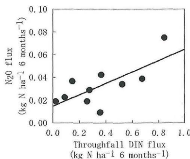
Fig. 5. The relationship between throughfall DIN and N 2 O flux.
