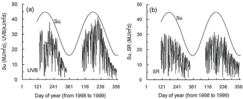
Fig. 1. Seasonal variations in UVB (a) and global solar radiation (b) with solar radiation at out of the earth's atmosphere in the Mountainous region of Nagano. Gaps for SR and UVB in figures show the periods when the sensors were being calibrated.
