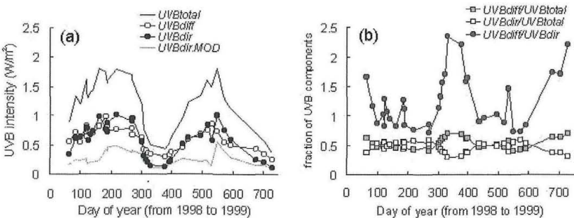
Fig. 5. Seasonal variations in the direct and diffuse UVB, and revised direct UVB as a function of SZA (a), and UVB_{diff}/UVB_{total} , UVB_{dir}/UVB_{total} and UVB_{diff}/UVB_{dir} (b).
