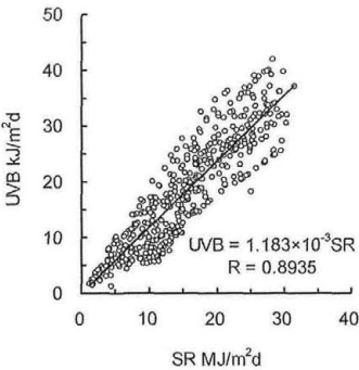
Fig. 4. Correlation between SR and UVB at Nagano.
