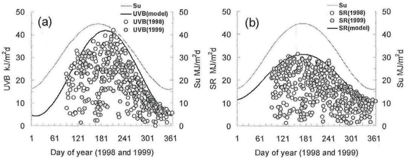
Fig. 2. Trend of seasonal variations for UVB and Su (a), and SR and Su (b). Figs. indicate measured value for UVB and Su in 1998 and 1999, and enveloped trends for these measured values (UVB(model) and SR(model)).
