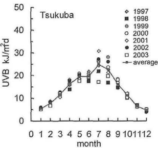
Fig. 3. Annual variations of UVB in Tsukuba. Solid line indicates 7years average.
