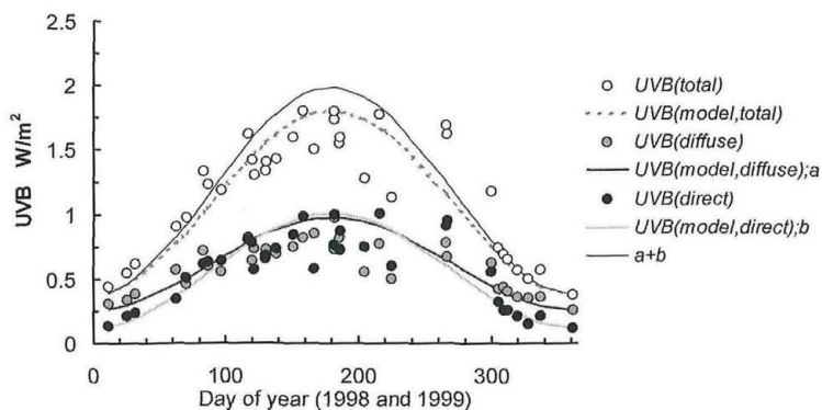
Fig. 6. Comparison of the measured and modelled values of direct, diffuse and total UVB measured at noon (JST) in 1998 and 1999.
