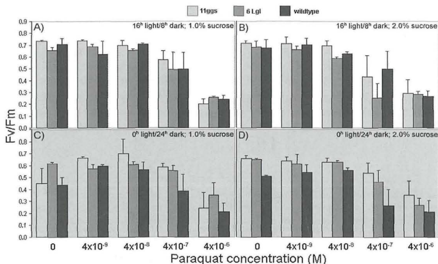
Fig. 2. Changes in the photosynthetic activity as characterized by chlorophyll fluorescence ( F_v/F_m ) in leaf discs of the wildtype poplar hybrid P. canadensis and its two genetically transformed lines (11ggs and 6Lgl) by different paraquat concentrations. The leaf discs were incubated in a 16 h light/8 h dark regime or in continuous darkness at 1.0 and 2.0 % external sucrose supplies in the solid medium. Means of 10 independent parallel experiments \pm standard deviations are shown.
