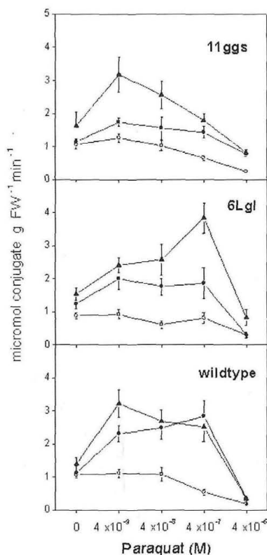
Fig. 1. Induction of glutathione S-transferase (GST) activity in leaf discs of the wildtype poplar hybrid P. canescens and its two genetically transformed lines (11ggs and 6Lgl) by different paraquat concentrations. The leaf discs were incubated in a 16 h light/8 h dark regime at three different external sucrose supplies in the solid medium. Symbols: \circ - 0.2 % sucrose; \bullet - 1.0 % sucrose; \blacktriangle - 2.0 % sucrose. Means of three independent parallel experiments \pm standard deviations are shown.
