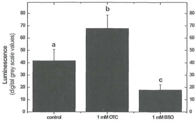
Fig. 4. Quantification of t-GSH in control, 1mM OTC and 1 mM BSO treated Cucurbita pepo L. leaf protoplasts. Luminescence, lead back to fluorescence, is represented as means of 20 to 30 replicate samples \pm standard deviation. Different letters (a, b, c) indicate significant differences ( P<0.01 ) analyzed by two-way analysis of variance (ANOVA).
