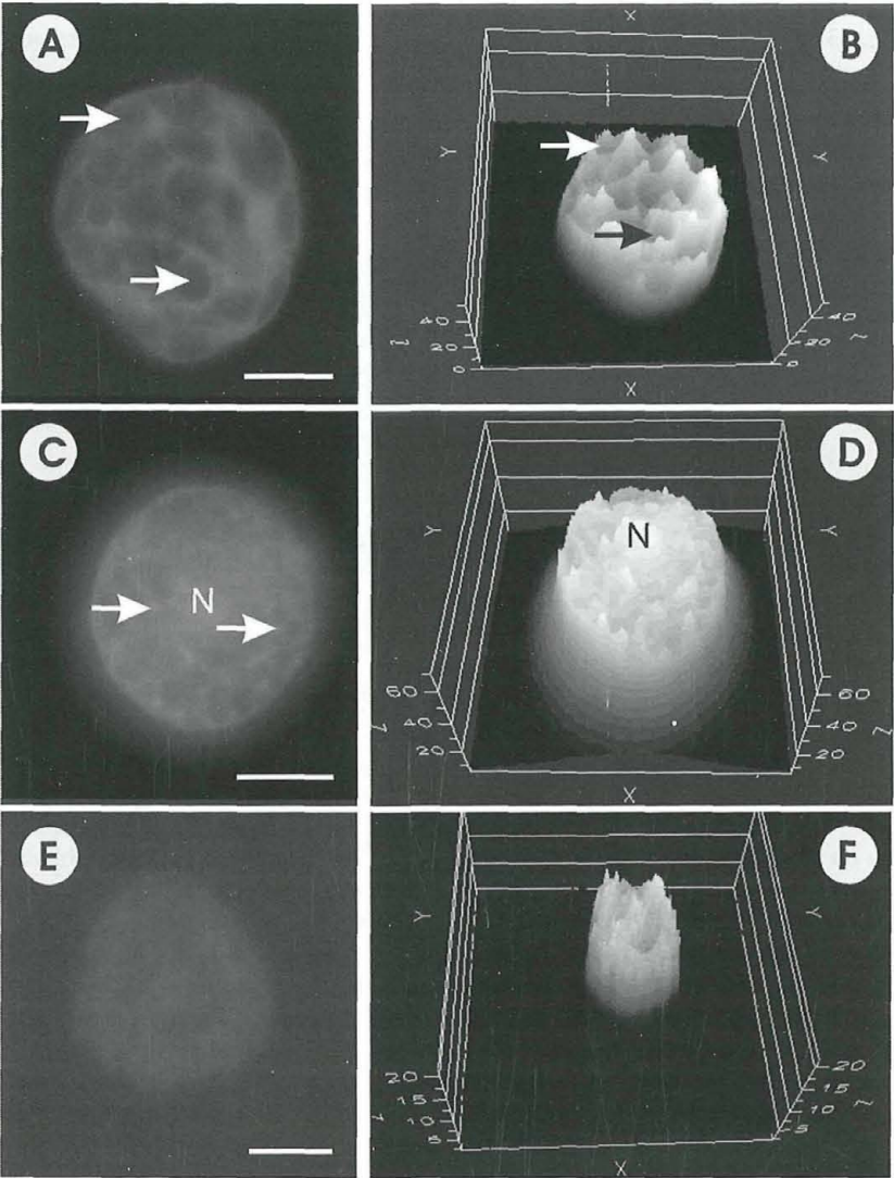
Fig. 3. Leaf protoplasts of Cucurbita pepo L. Immunofluorescence images (A, C, E) and appropriate luminescence profiles (B, D, F). (A, B) Untreated protoplasts showing positive fluorescence in cytoplasm. Chloroplasts are not stained (arrows). (C, D) 1 mM OTC treated cell is characterized by stronger fluorescence in cytoplasm and in nucleus (N). Mitochondria are visible as bright fluorescence dots (arrows). (E, F) Treatment with 1 mM BSO leads to very poor fluorescence image. Bars = 20 μm.
