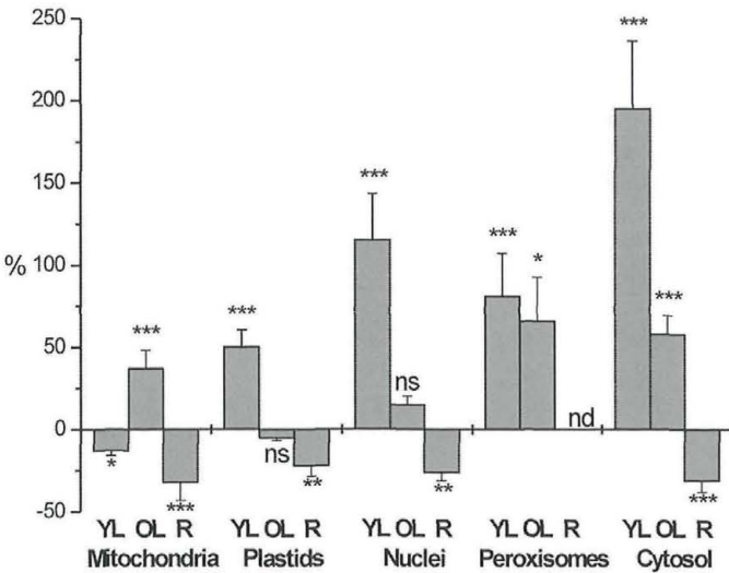
Fig. 6. Statistica graph showing the distribution of t-GSH in ZYMV-infected leaf mesophyll and root tip cells in comparison to the control. Values are means \pm standard deviation and document the percentage of increase or decrease in the amount of gold particles bound to glutathione. nd=not determined; n > 20 for peroxisomes and n > 60 for other cell structures. Significant differences between organelles of control and organelles of ZYMV-infected cells were calculated with the Mann Whitney U-test. ns if p > 0.05 , (*) if p < 0.05 , (**) if p < 0.01 , and (***) if p < 0.001 ; YL=younger leaves, OL= older leaves and R=roots.
