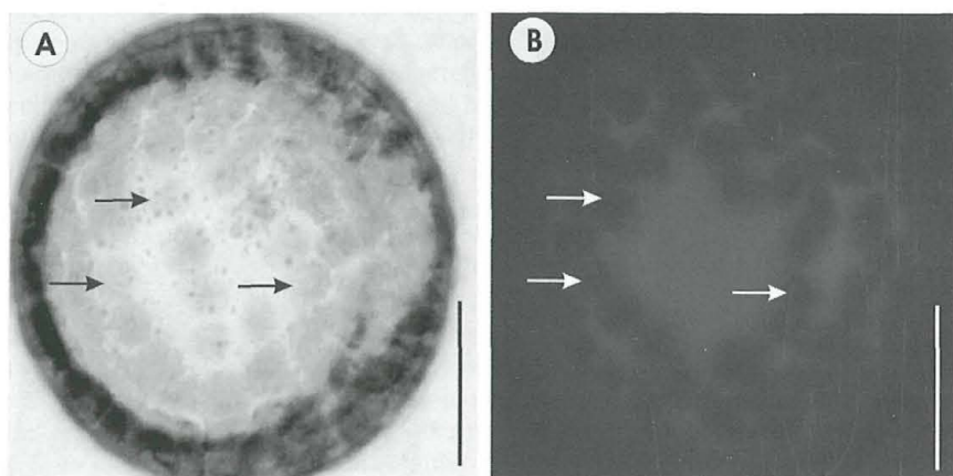
Fig. 2. Leaf protoplast of Picea abies L. Bright field (A) and BmCl fluorescence image (B). (A) Bright field image showing roundish protoplast with chloroplasts (arrows). (B) Fluorescence picture showing positive fluorescence in cytoplasm. Chloroplasts are not stained (arrows). Bars = 20 \mu m.
