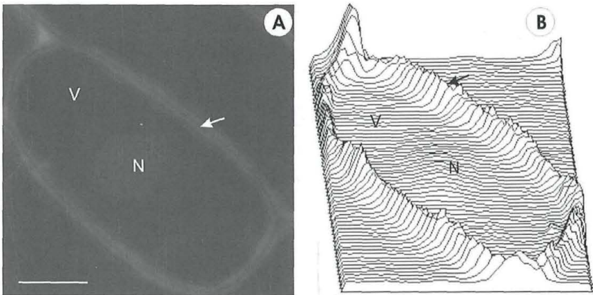
Fig. 1. Epidermal cell of Allium cepa L. BmCl Fluorescence image (A) and appropriate luminescence profile (B). (A, B) Epidermal cell showing positive fluorescence in cytoplasm and nucleus (N); no fluorescence could be observed in cell wall (arrow) and vacuole (V). Bar = 20 \mu m.
