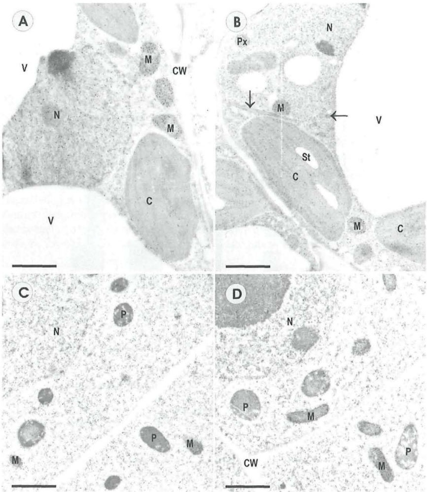
Fig. 5. Transmission electron micrographs of leaf mesophyll and root tip cells with immunogold labeling of glutathione. Cells from sections, taken from the center of the leaves and from root tips fixed for immunogold labeling and post stained for 15 sec. with uranyl acetate. Bars=1 \mu m. A) Control cells of younger leaf showing gold particles in chloroplasts (C), mitochondria (M), the nucleus (N) and the cytosol. B) ZYMV-infected cells of younger leaf with cylindrical inclusions (arrows) in the cytosol and gold particles in mitochondria (M), peroxisome (Px), the nucleus (N) and chloroplasts (C) with starch (St). C) Control root tip cells showing gold particles in mitochondria (M), plastids (P), the nucleus (N) and within the cytosol. D) ZYMV-infected root tip cells with gold particles in plastids (P), mitochondria (M), the nucleus (N) and the cytosol. In general no or only few gold particles bound to glutathione were found in cell walls (CW) and vacuoles (V) within root tip and leaf mesophyll cells.
