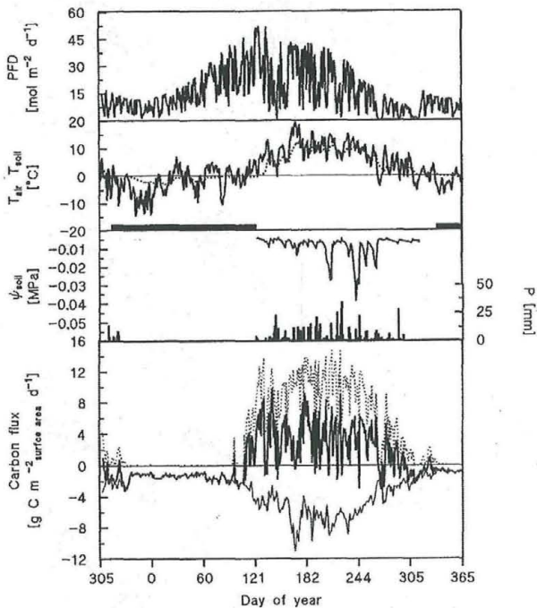
Fig. 2. Time course of daily sum of photon flux density (PFD), daily mean air ( T_{\text{air}} , solid line) and soil temperature at 5 cm soil depth, ( T_{\text{soil}} , dotted line) winter snow cover (solid area), soil water potential ( \Psi_{\text{soil}} ), daily sum of precipitation (P), as well as daily net ecosystem production (NEP; thick solid line), ecosystem respiration (ER; thin solid line), and gross primary production (GPP; thin dotted line) in the Pinus cembra ecosystem under study between November 5, 2001 and December 31, 2002.
