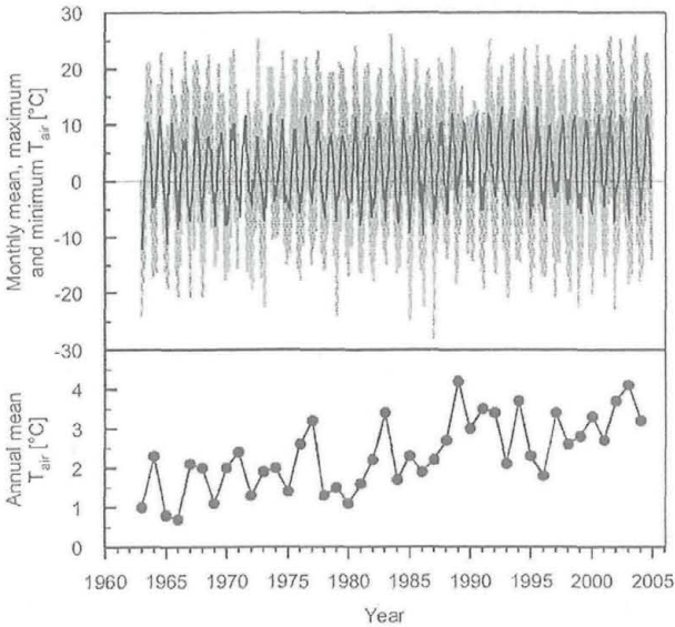
Fig. 4. Variation in monthly mean, maximum and minimum air temperature (top), and changes in annual mean air temperature (bottom) from January 1963 throughout December 2004 at the Klimahaus Research Station, 1950 m a.s.l. (Mt. Patscherkofel, Innsbruck, Austria).
