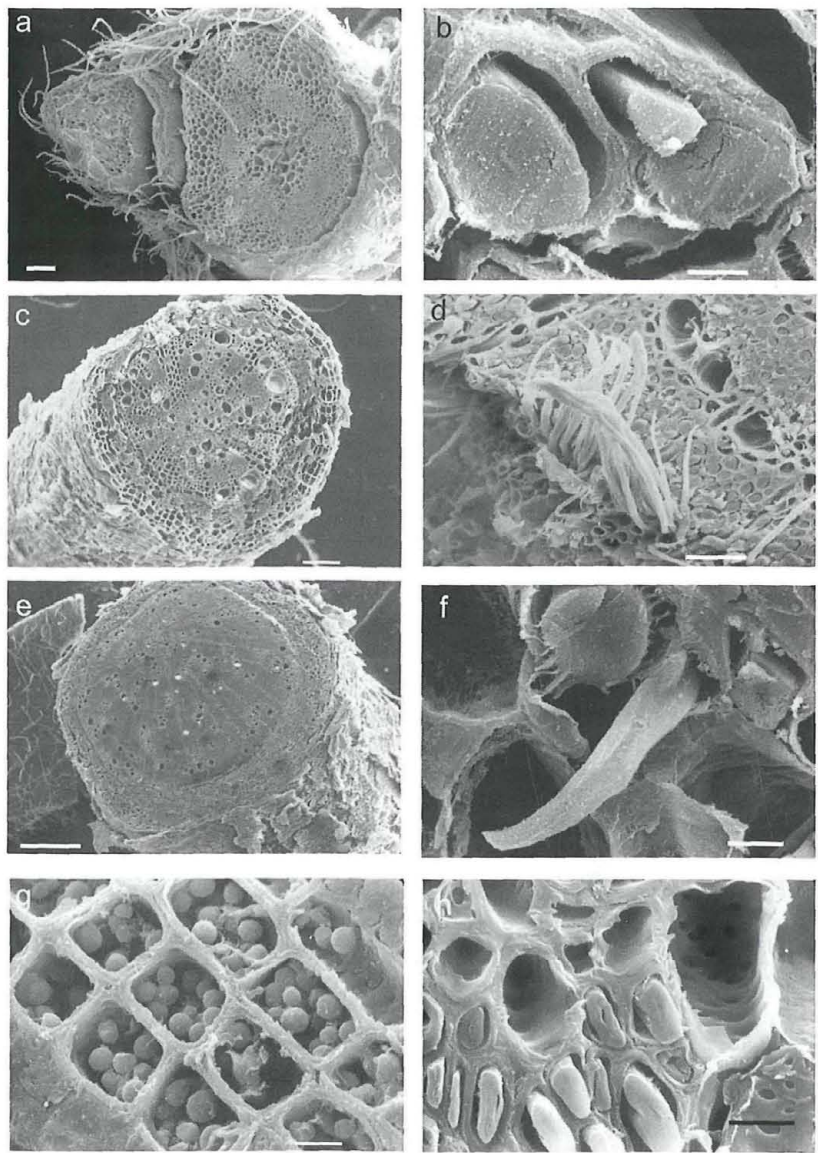
Fig. 3. The "woody" vegetative stage (SEM micrographs). a. vegetative bud from half-hardy stem (cross section), bar: 10 µm; b. fibres in woody stem, bar: 1 µm; c. main root (cross section), bar: 100 µm; d. fibres in the tap root (uncompleted cross section), bar: 10 µm; e. woody stem (cross section), bar: 50 µm; f. fibres (gelatinous?) from woody stem, bar: 2 µm; g. storage (reserve) starch grains in the ray parenchyma of woody stem, bar: 10 µm; h. integrate tracheary elements in woody stem, bar: 10 µm.
