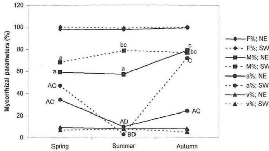
Fig. 6. Mycorrhizal colonization parameters for transplanted (SW) and control (NE) B. pinnatum roots in the two exposures of site M in 2002. Samples were taken in spring (May), summer (August) and autumn (October). Statistically significant differences among treatment means (or medians for non-parametric data) of 5 replicates are indicated with lowercase letters next to symbols. Different letters indicate significant differences ( P < 0.05 ). F%: frequency of mycorrhizal colonization. M%: intensity of mycorrhizal colonization. a%: arbuscule content. v%: vesicle content. For explanation of mycorrhizal parameters see the Material and Methods section. On M% data two-way ANOVA was performed. On a% data Kruskal-Wallis test and Dunn's test was used. Means of treatments in the case of F% and v% did not differ significantly (data not shown).
