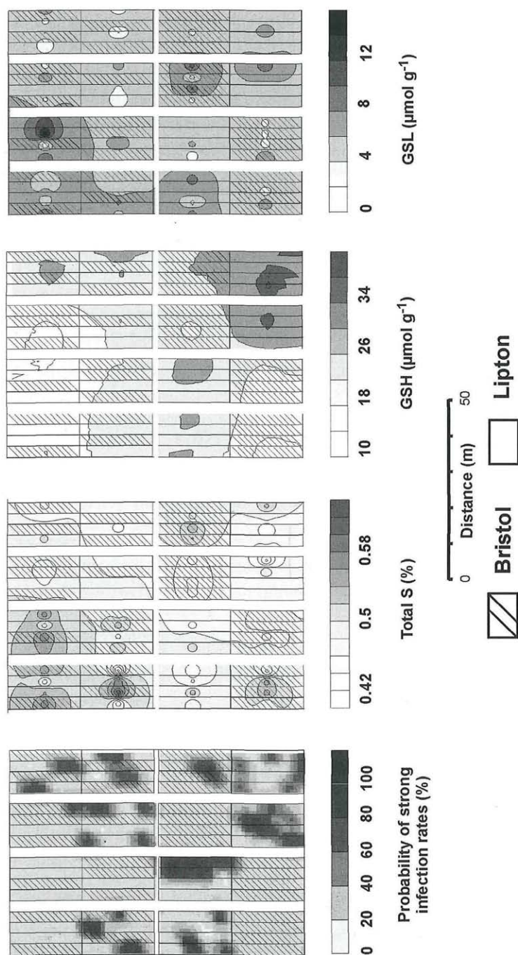
Fig. 2. Small-scale spatial variability of the probability of severe infections of oilseed rape with L. maculans , glutathione, glucosinolate, and total S content.
