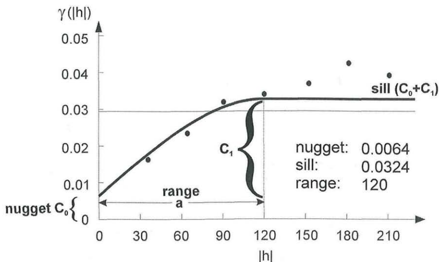
Fig. 1. Example for a spherical (semi)variogram model.
