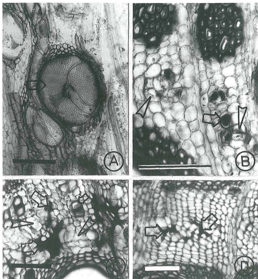
Fig. 3. Tangential (A) and transverse (B–D) view of xylem and included phloem in the stem of Canavalia ensiformis (L.) DC.
