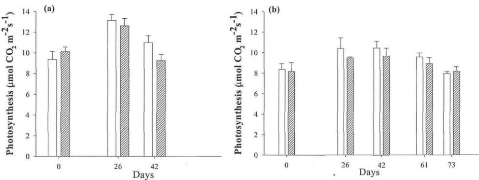
Fig. 1. Effects of \text{O}_3 on the rate of photosynthesis ( \mu\text{mol m}^{-2} \text{ s}^{-1} ) in cvs. (a) Bogota and (b) Elsanta. Measurements were made on the 1 st or 2 nd most recent fully expanded leaf. Values are means ( \pm \text{SE} ) of 9 or 13 replicate plants for Bogota and 4 replicate chambers for Elsanta. Open bars represent plants exposed to filtered air, hatched bars represent plants exposed to ozone.
