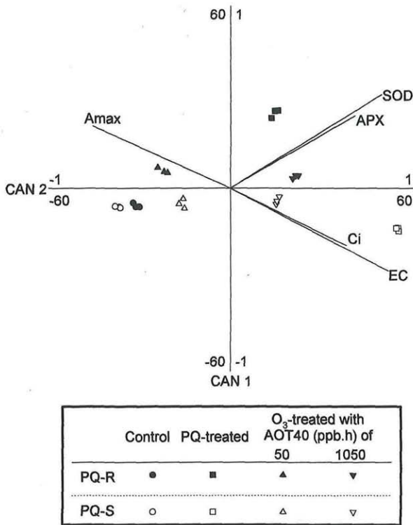
Fig. 2. Ordination biplot of biochemical and physiological parameters (vectors) under four paraquat and ozone treatments (one control, two ozone regimes, one paraquat spray) of the two Conyza bonariensis biotypes. CAN 1, first canonical variable; CAN 2, second canonical variable. Each point represents the mean value of each replicate test. For abbreviations, see caption of Fig. 1.
