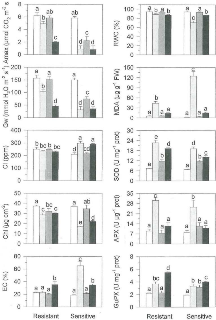
Fig. 1. Effect of paraquat and ozone treatment and of genotypical variation on photosynthetic parameters, membrane state and antioxidant enzymes of the two biotypes of Conyza bonariensis . Legend: white = control; grey = PQ-treated plants; dark grey = O 3 -treated plants (AOT40 50 ppb.h); black = O 3 -treated plants (AOT40 1050 ppb.h). Abbreviations: A max = photosynthetic activity at saturating light; APX = ascorbate peroxidase; Chl = total chlorophylls; Ci = intercellular CO 2 concentration; EC = electrical conductivity of leachates from foliar discs, expressed in percentage of control discs which have been frozen to disrupt membrane integrity; GuPX = guaiacol peroxidase; Gw = stomatal conductance to water vapor; MDA = malondialdehyde; RWC = relative water content; SOD = superoxide dismutase. Vertical bars over each column indicate standard deviation; in each graph, columns marked with the same letters are not different for P ≤ 0.05.
