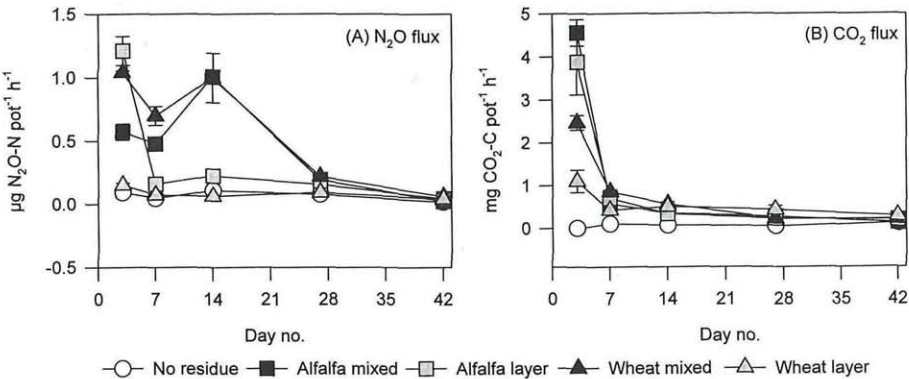
Fig. 3. Fluxes of N 2 O and CO 2 from incubated soil with alfalfa and wheat crop residues with different placements. Each datapoint is a mean of n=3±SE.
