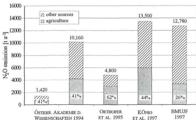
Fig. 1. Estimates of Austrian \text{N}_2\text{O} emissions.
