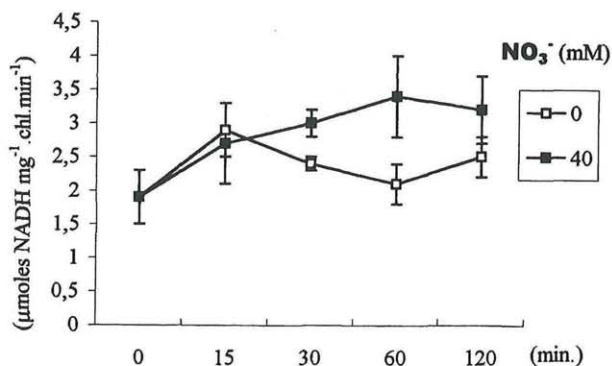
Fig. 3. Effect of 40 mM \text{KNO}_3 on PEPCase activity of detached maize leaves. The leaves were detached from N-limited plants after a 16 h period in darkness and transferred to 0 or 40 mM \text{KNO}_3 nutrient solutions in the light ( 1000 \mu\text{mol m}^{-2} \text{s}^{-1} ), for up to 2 h. Each point is the mean \pm SE ( n \geq 3 )
