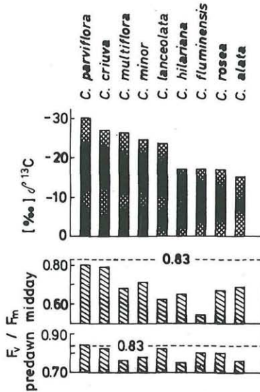
Fig. 6. Acute and chronic photoinhibition given by measurements of potential quantum yield of photosystem II ( F_v/F_m ) for several species of Clusia at midday after short periods of dark adaptation (acute photoinhibition at times of the day when CAM plants are in phase III) and before dawn after the nocturnal dark period. Data are averages from the literature on measurements in the field as well as in the laboratory. The species are arranged from left to right according to increasing (decreasingly negative) carbon isotope ratios ( \delta^{13}\text{C} ) which indicate dominant \text{C}_3 -photosynthesis on the left hand and dominant CAM on the right hand of the distribution and \text{C}_3/\text{CAM} intermediate behaviour in between. (After LÜTTGE 1999)
