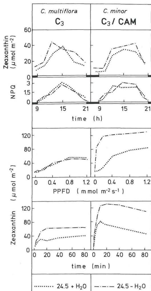
Fig. 8. Daily courses of zeaxanthin levels and thermal energy-dissipation (non-photochemical fluorescence quenching, NPQ) in the plants of C. multiflora and C. minor shown also in Fig. 7 on day 5 after transfer to high daily light doses ( 24.5 \text{ mol m}^{-2} \text{d}^{-1} ) with and without drought stress as indicated (2 upper panels). Lower panels show short term experiments with C. multiflora and with C. minor in the CAM-state where photosynthetic photon flux density (PPFD) was presented for 20 min, as indicated, or a PPFD of 1000 \mu\text{mol m}^{-2} \text{s}^{-1} was given for various times up to 80 min, as indicated, before analysis of zeaxanthin levels. (After HERZOG & al. 1999).
