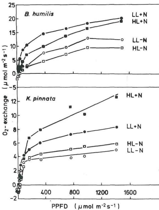
Fig. 3. Light-dependence of \text{O}_2 -evolution of leaf samples of Bromelia humilis (after FETENE & al. 1990) and Kalanchoë pinnata (after LÜTTGE & al. 1991b) grown at high light (HL) and low light (LL) with (+N) and without (-N) nitrogen supply.
