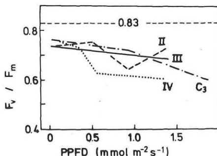
Fig. 5. Light-response characteristics of acute photoinhibition given by measurements of potential quantum yield of photosystem II ( F_v/F_m ) in plants of the \text{C}_3/\text{CAM} intermediate species Clusia minor in the \text{C}_3 -state ( \text{C}_3 ) and in the CAM-state during phases II, III and IV of CAM. Plants were kept at the photosynthetic photon flux densities (PPFD) indicated and darkened for 10 min before F_v/F_m was determined. (After HAAG-KERWER 1994.)
