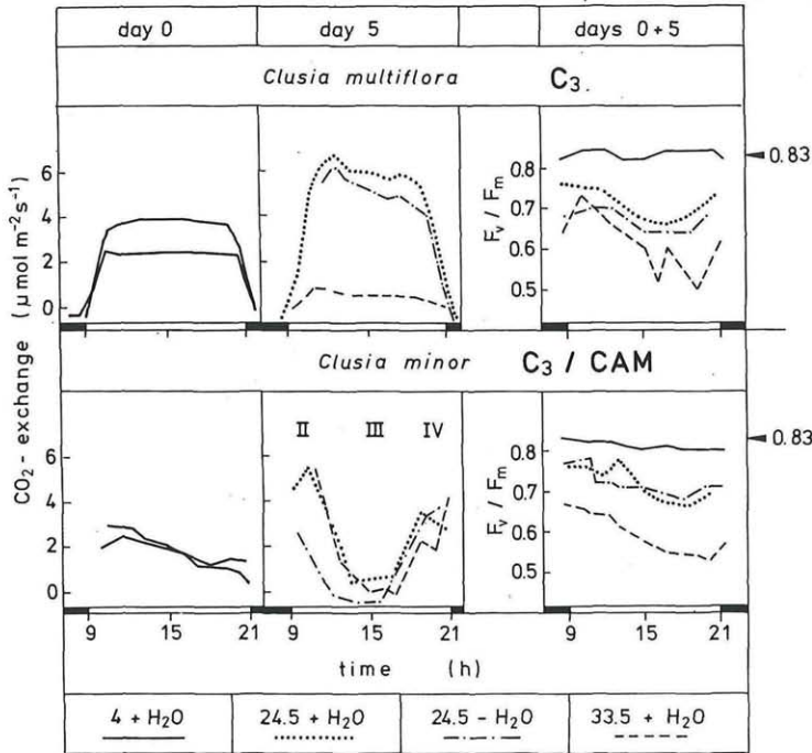
Fig. 7. \text{CO}_2 -exchange and photoinhibition given by measurements of potential quantum yield of photosystem II ( F_v/F_m ) in the \text{C}_3 -species Clusia multiflora and the \text{C}_3/\text{CAM} -intermediate species Clusia minor . Plants were grown at low light and after day 0, the last day at low light, they were transferred to two different high daily light doses applied in a bell-shaped time course (not shown) with additional stress due to withholding water in one case. The behaviour on day 0 (solid lines) and 5 days after the transfer (other lines) is shown; numbers at the bottom of the graph explaining the lines are daily doses of photosynthetic photon flux density ( \text{mol m}^{-2} \text{d}^{-1} ); roman numbers for gas exchange of C. minor on day 5 indicate CAM phases. (After HERZOG & al. 1999)
