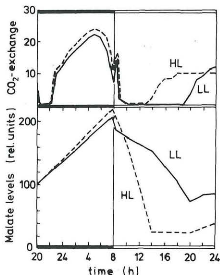
Fig. 4. \text{CO}_2 -exchange and malate levels in phyllodia of plants of Kalanchoë tubiflora grown at low light and measured in the light period (open bar on abscissa) following the dark period (dark bar on abscissa) shown at the same low light intensity as experienced during growth (LL) and at a much higher (2.4-fold) light intensity (HL), respectively. (After KLUGE 1968.)
