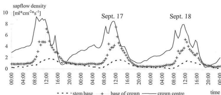
Fig. 5. Diurnal course of sap flow in different stem parts of sample tree A1 during advanced drought stress, Sept. 16th - Sept. 18th 1997.
