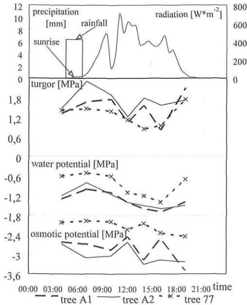
Fig. 2. Diurnal course of the parameters of water status on June 3rd 1998, after a three-week drought: turgor, water potential and osmotic potential, compared to precipitation and radiation (above); arrow: a 6.4 mm rain shower at 04:30 a.m., just before sunrise. For explanation of tree no. see legend in fig.1.
