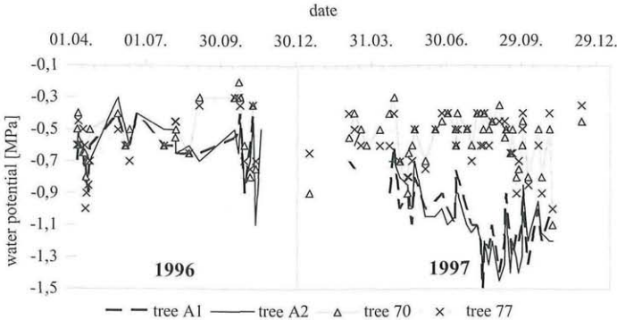
Fig. 1. Course of pre-dawn water potential in the upper crown of sample trees A1 and A2 submitted to conditions of prevention water supply, reference tree 70 (heavily damaged) and healthy reference tree 77, during 1996 and 1997.
