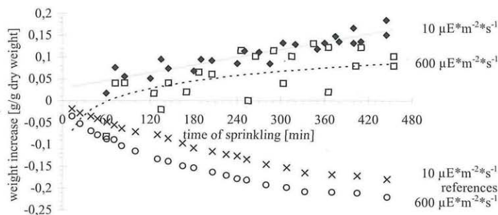
Fig. 3. Course of weight increase of detached permanently sprinkled needles; the low light variant ( \blacklozenge ) shows a linear increase, the light variant ( \square ) a moderate increase with high deviation; comparison with the reference without sprinkling: ( \circ ) for 600 \mu\text{E m}^{-2} \text{s}^{-1} and ( \times ) for 10 \mu\text{E m}^{-2} \text{s}^{-1} .
