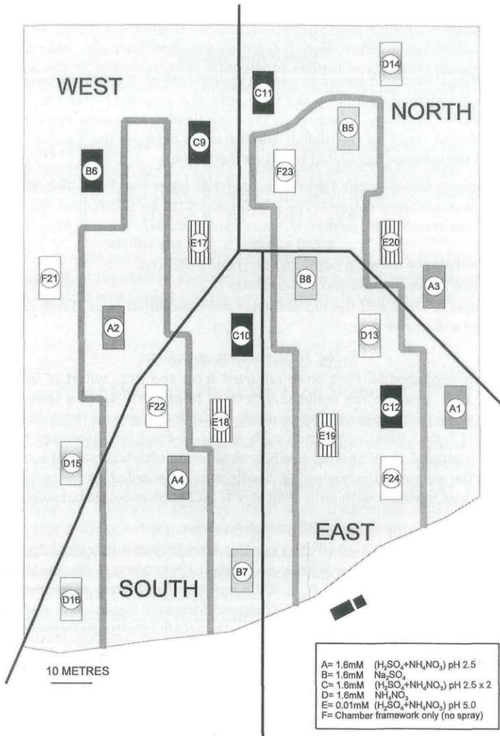
Fig. 1. Layout of the six experimental treatments (A–F) used to examine the effects of N, S and acid inputs on the vitality of Sitka spruce. The site is divided into 4 blocks (see solid black lines) designated south, west, north and east. The hatched continuous lines represent brashed walkways leading into the experimental area and out again. Each treatment chamber is represented once per block as 10 trees arranged in 2 parallel lines of 5 trees, surrounded by a scaffolding framework supporting the spray facility. Treatment E represents the control, a dilute salt solution at the pH of the rain water (~ 4.8), treatment F with no spray will be used to evaluate the impact of additional rainwater. Treatments B and D enable effects of S and N in the absence of acidity to be assessed and A and C provide acidified (pH 2.5) N and S at a single (*) and double dose (*2).
