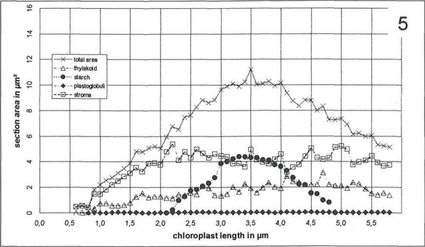
Fig. 5. Areas of the different structural components within chloroplast 5 of Figs. 1, 2.
