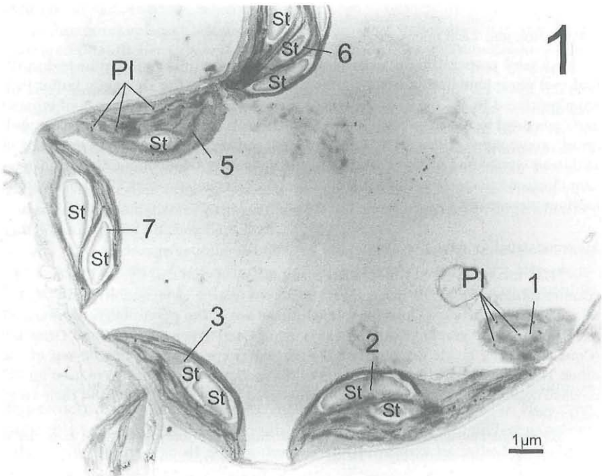
Fig. 1. TEM-micrograph of a spinach mesophyll cell used for 3 D reconstruction. Scale bar = 1 \mu m.
