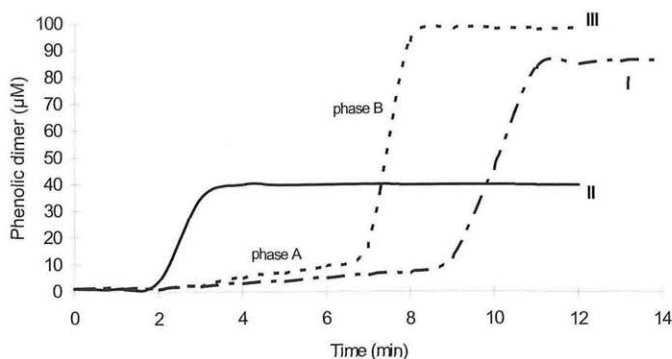
Fig. 2. (I) Schematic presentation of the biphasic behavior of peroxidase mediated phenol and thiol oxidation of the in vitro system horseradish peroxidase (7 nM)/cysteine (25 μM)/homovanillic acid (500 μM). During phase A all thiol is oxidized (accompanied by oxygen consumption), whereas during phase B phenol is oxidized following the classical peroxidase pathway [reactions (1), (8) and (9)]. At high (0.1 μM) enzyme concentrations (II) the system becomes monophasic. Necessary hydrogen peroxide derives from reactions happening during phase A. Superoxide dismutase (Cu/Zn 150 units) shortens phase A and increases the amount of H-A-A-H [III, enzyme as in I].
