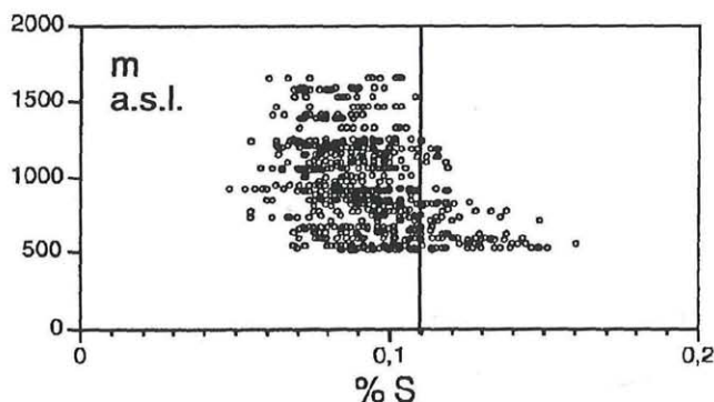
Fig. 10. Total sulphur content of individual sample plots, depending on altitude (needle year 1, 1983-1992).
