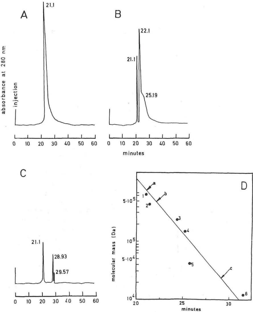
Fig. 2. Chromatographic traces in SE-HPLC corresponding to fractions I (A), II (B) and III (C) eluted from Sephadex G-150 column. Estimation of molecular weight (D) of ferritin-glutaraldehyde-ferritin (a), ferritin-glutaraldehyde-arginase (b) and free arginase (c) where standards were 1= tyroglobulin (660 kDa), 2 = apoferritin (450 kDa), 3 = catalase (240 kDa), 4 = alcohol dehydrogenase (160 kDa), 5 = egg albumin (44 kDa) and 6 = cytochrome c (12.5 kDa)
