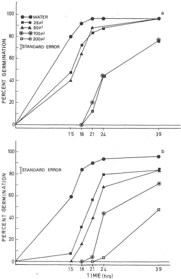
Fig. 1: The effect of various volumes of phase I (a) and phase II (b) at the concentration of 0.3 endosperm/ \mu l on the germination of Lactuca sativa var. Great Lakes. Each point is the mean of three replications.
