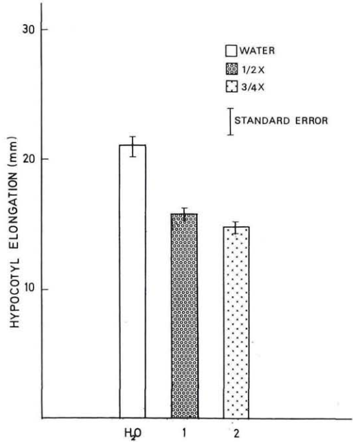
Fig. 6: The effect of various concentrations of the active peak of fraction 5 on the hypocotyl elongation of Lactuca sativa var. Great Lakes. Values expressed as mean \pm SE.
