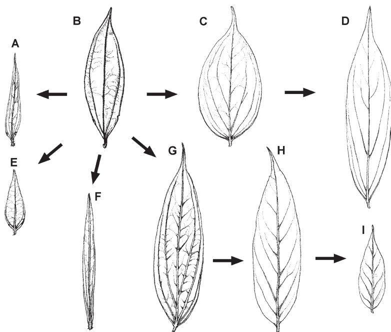
Fig. 3. Leaf shape and size of various taxa in Vaccinium section Rigiolepis . Venation is camptodromous and the arrows suggest possible routes to either blade contraction or expansion. A. Vaccinium minimiflorum ; B. V. suberosum ; C. V. megaphyllum ; D. V. leptanthum ; E. V. uniflorum ; F. V. linearifolium ; G. V. acuminatissimum ; H. V. moulinii ; I. V. andersonii .
