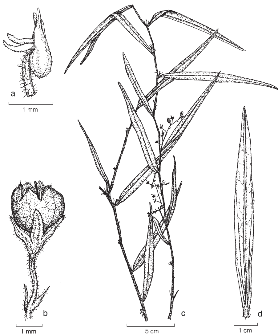
Fig. 6. Vaccinium linearifolium Klotz. a. Stamen; b. flos; c. ramus; d. folia (all: Yii S 55984 in 1988 (L.) depictum est).
