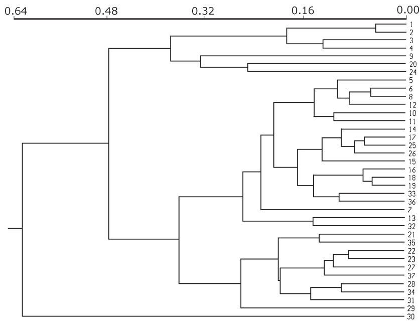
Fig. 1. Phenogram depicting clusters when characters 16 and 17 are read sensu lato, i.e., the bracts and calyx lobes are ribbed as in V. crinigrum (Fig. 5c).
