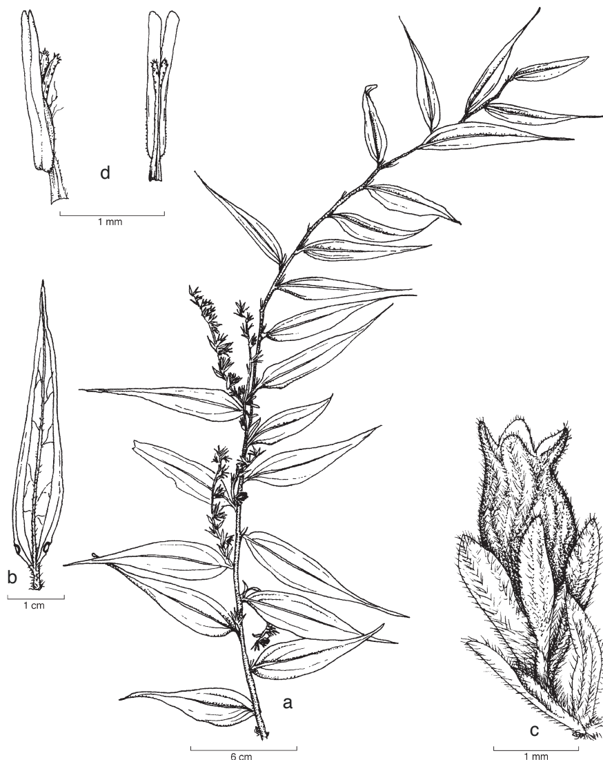
Fig. 5. Vaccinium crinigrum Kloeke. a. Ramus; b. folia; c. flos; d. stamen (all: Burt & Woods B2781 in 1962 (L) depictum est).
