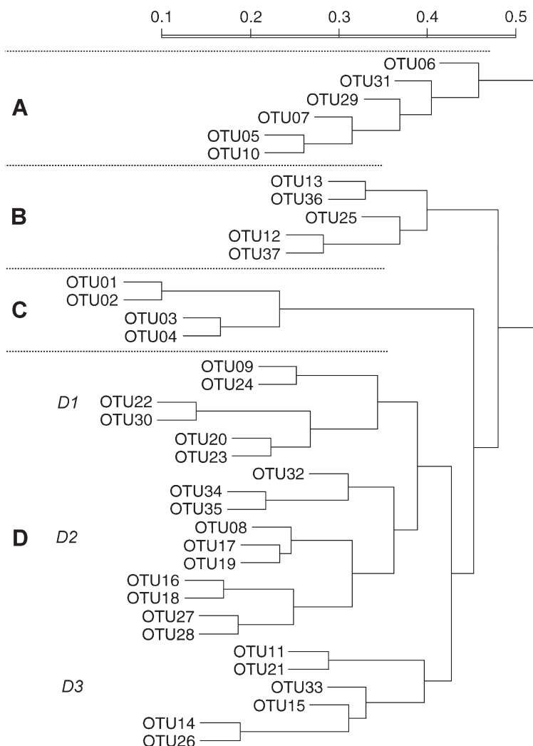
Fig. 2. Phenogram depicting clusters when characters 16 and 17 are read sensu stricto, i.e., the bracts and calyx lobes are 'not or but indistinctly ribbed' in V. crinigrum .
