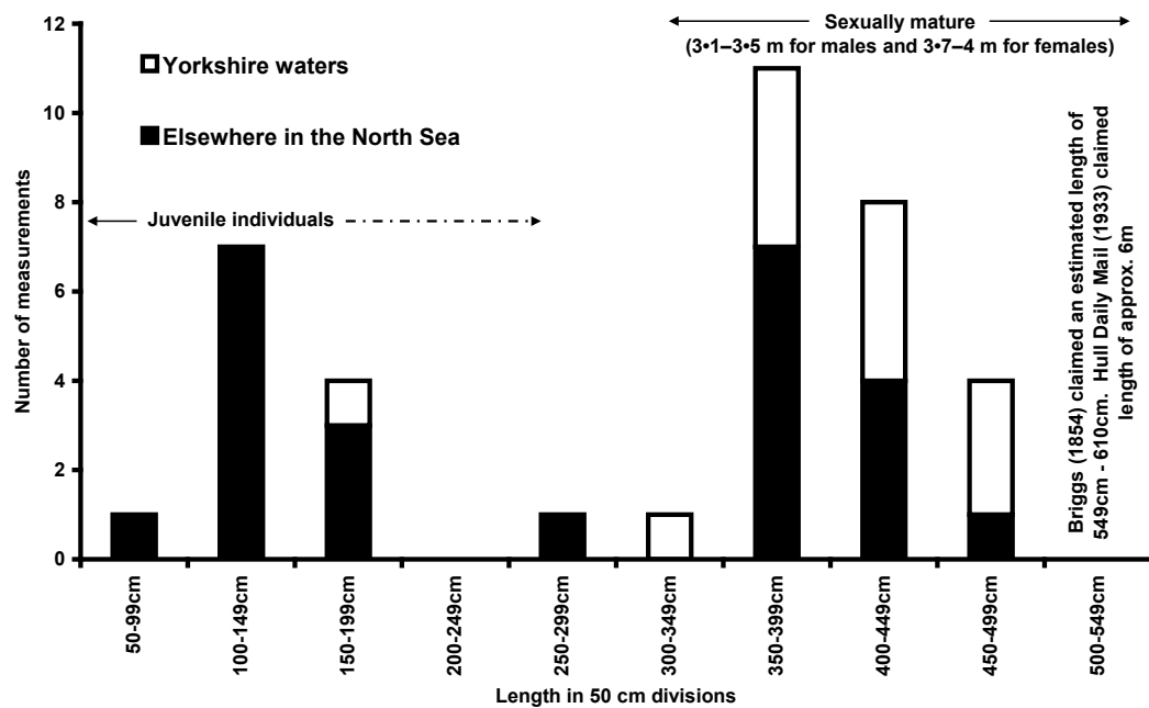
Figure 3: Claimed lengths (in 50cm divisions) of North Sea and Yorkshire coast records.
