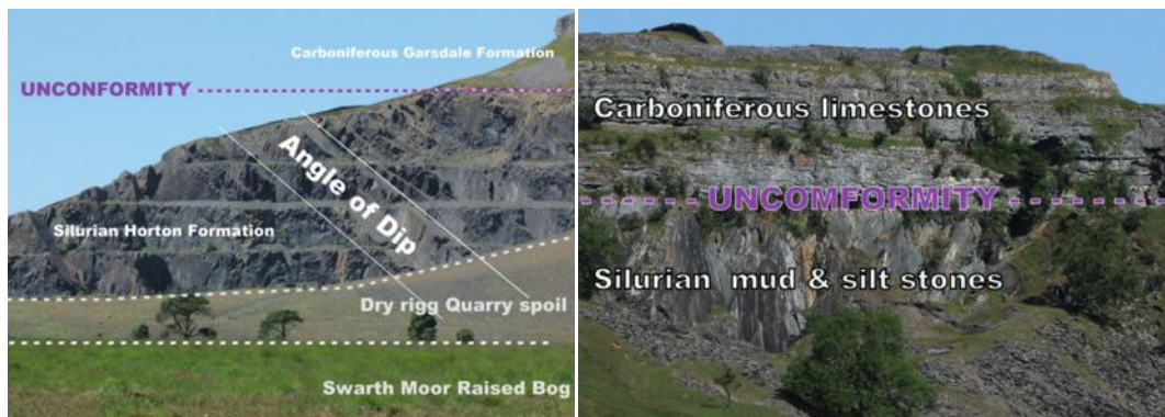
Figure 6 (see p214). Dry Rigg Quarry and Arcow Quarry activities over the years have revealed a spectacular Silurian/ Carboniferous unconformity.
