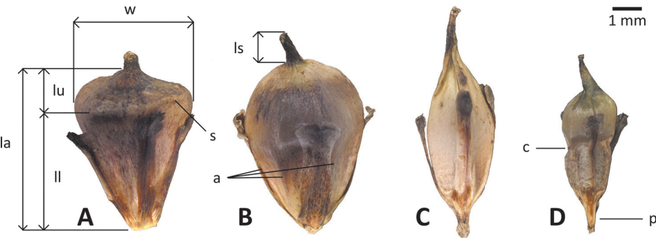
Fig. 1. – Morphological characters of fruit: (A) Sparganium erectum subsp. erectum ; (B) S. e. subsp. oocarpum ; (C) S. e. subsp. neglectum ; (D) S. e. subsp. microcarpum . Scale bars: 1 mm. a – number of angles; c – constriction; la – length of fruit; ll – length of the lower part of fruit; lu – length of upper part of fruit; ls – length of style; p – peduncle; s – shoulder between upper and lower parts; w – width of fruit. Photo S. Pířová.
