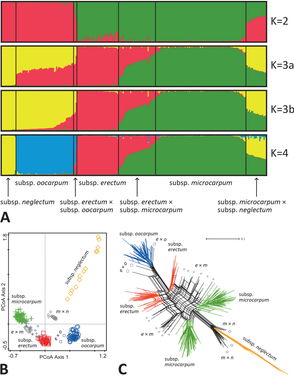
Fig. 2. – Results of molecular analyses of 242 individuals of Sparganium erectum based on 103 AFLP loci: (A) Bar plot showing Bayesian assignment probabilities using software STRUCTURE for two, three and four clusters ( K = 2-4 ). The genetic groups (containing individuals with < 15\% admixture with another group) associated with subspecies were recorded plus intermediate individuals between them. (B) Principal coordinate analysis (PCoA) using Jaccard's similarity coefficient. The first and second axis explained 25.5% and 14.8% of the variation, respectively. (C) Neighbour-Network. Colours indicate AFLP groups detected by STRUCTURE.
