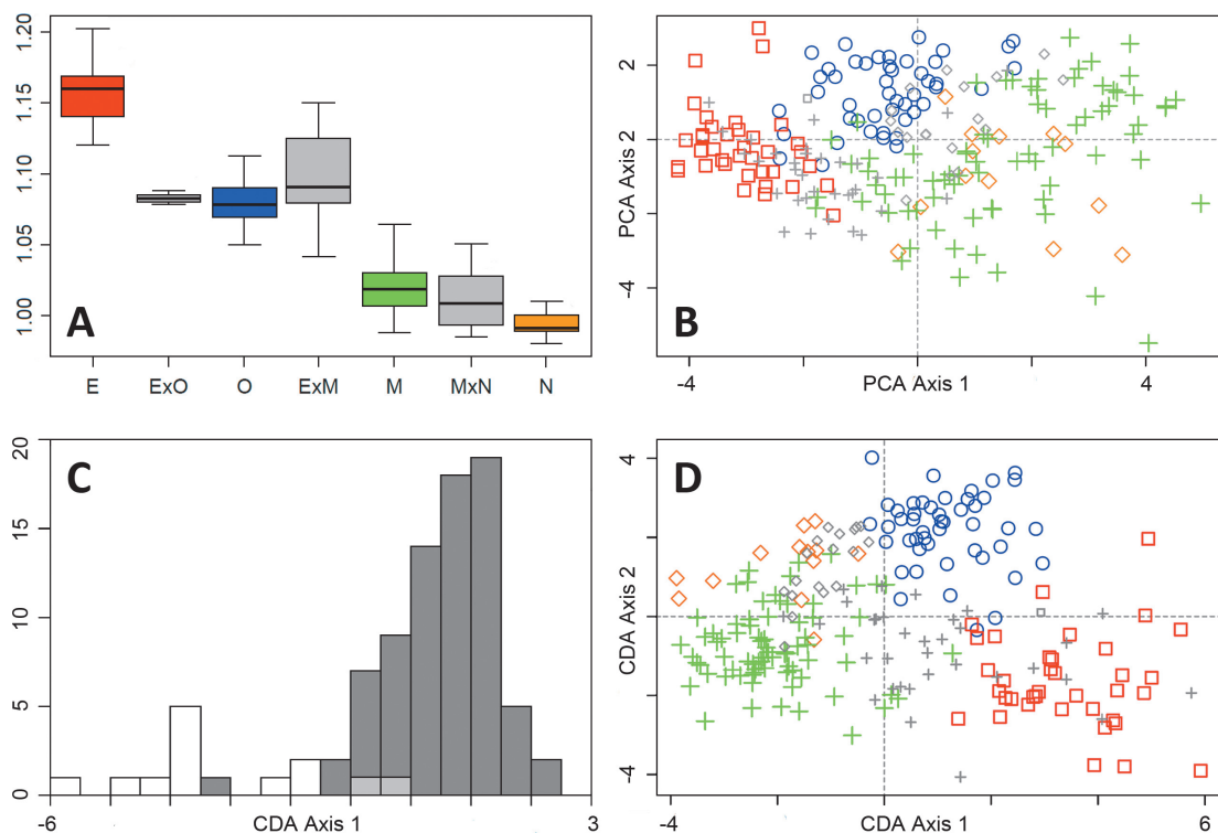
Fig. 4. – (A) Box plot showing the intraspecific distribution of genome size in Sparganium erectum (N = 223). The admixed groups are in grey boxes. E: subsp. erectum , ExO: subsp. erectum × subsp. oocarpum , O: subsp. oocarpum , ExM: subsp. erectum × subsp. microcarpum , M: subsp. microcarpum , MxN: subsp. microcarpum × subsp. neglectum , N: subsp. neglectum . (B) Principal component analysis (PCA) based on 12 morphological characters of the fruit of 227 individuals of Sparganium erectum . The first and second axis explained 42.0% and 20.6% of the variation, respectively. (C) Canonical discriminant analysis (CDA) of 77 individuals of subsp. microcarpum (dark grey columns) and 13 individuals of subsp. neglectum (white columns) with the overlap between both (light grey columns). (D) Canonical discriminant analysis (CDA) of 227 individuals of S. erectum based on 12 morphological characters of fruit. The first and second components explained 43.1% and 35.9% of the variation, respectively. Colours indicate AFLP groups detected by STRUCTURE and passively projected admixed individuals: ◻ subsp. erectum ; ◯ subsp. oocarpum ; + subsp. microcarpum ; ◊ subsp. neglectum ; ◻ subsp. erectum × subsp. oocarpum ; + subsp. erectum × subsp. microcarpum ; ◊ subsp. microcarpum × subsp. neglectum .
