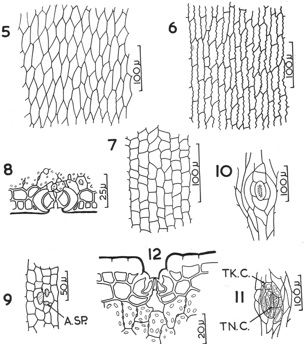
Figs. 5—7. ADAXIAL EPIDERMIS, SURFACE VIEW. 5, Ptychosperma Macarthurii ; 6, Cyrtostachys Lakka ; 7, Coccothrinax argentea ; 8, Phoenix canariensis , t.s. stoma; 9, Phoenix canariensis , hypodermis, surface view, with substomatal cells; 10, Caryota mitis , stoma, surface view; 11, Caryota mitis , base of epidermal hair, surface view; 12, Sabal mexicana , t.s. stoma. —a. sp.—intercellular air-space; tk. c.—thick-walled cells; tn. c.—thin-walled cells.
