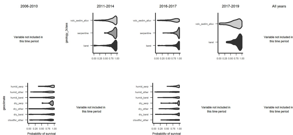
Fig 9. Marginal plots of geological substrate and geoclimate zones through time. Class names are in see Table 3.
