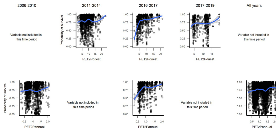
Fig 8. Marginal plots through time of long-term potential evapotranspiration to precipitation ratio for the year (PET2Pannual) and the driest quarter (PET2Pdriest). This index is inversely related to aridity.
