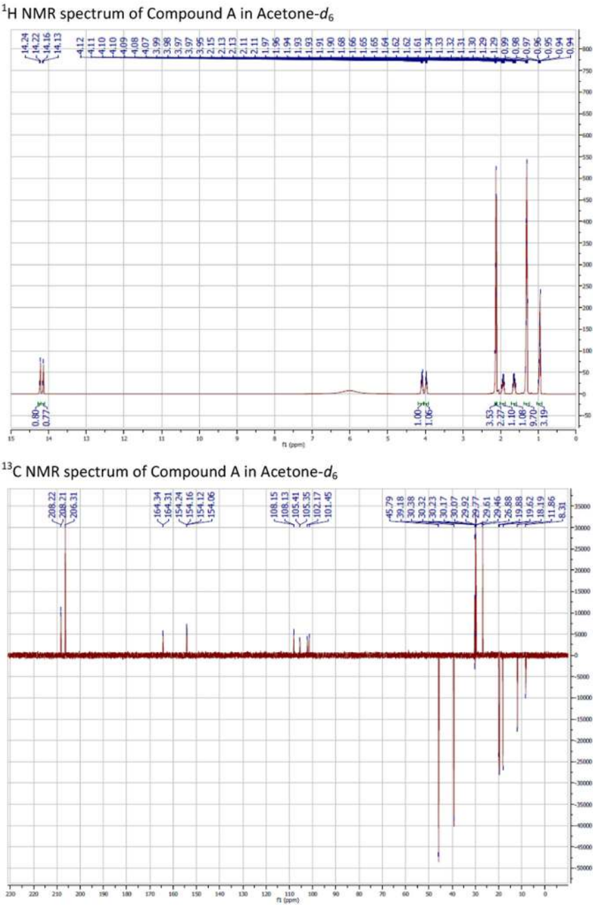
Fig. 1. NMR spectra of compounds.
