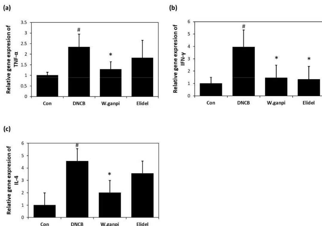
Figure 5. Effects of WGE on the relative gene expression of cytokines TNF- \alpha , IFN- \gamma , and IL-4 in DNCB sensitized mouse dorsal skin. (a) The mRNA expression of TNF- \alpha ; (b) The mRNA expression of IFN- \gamma ; (c) The mRNA expression of IL-4. # p < 0.05 vs. the CON group; * p < 0.05 vs. the DNCB group.
