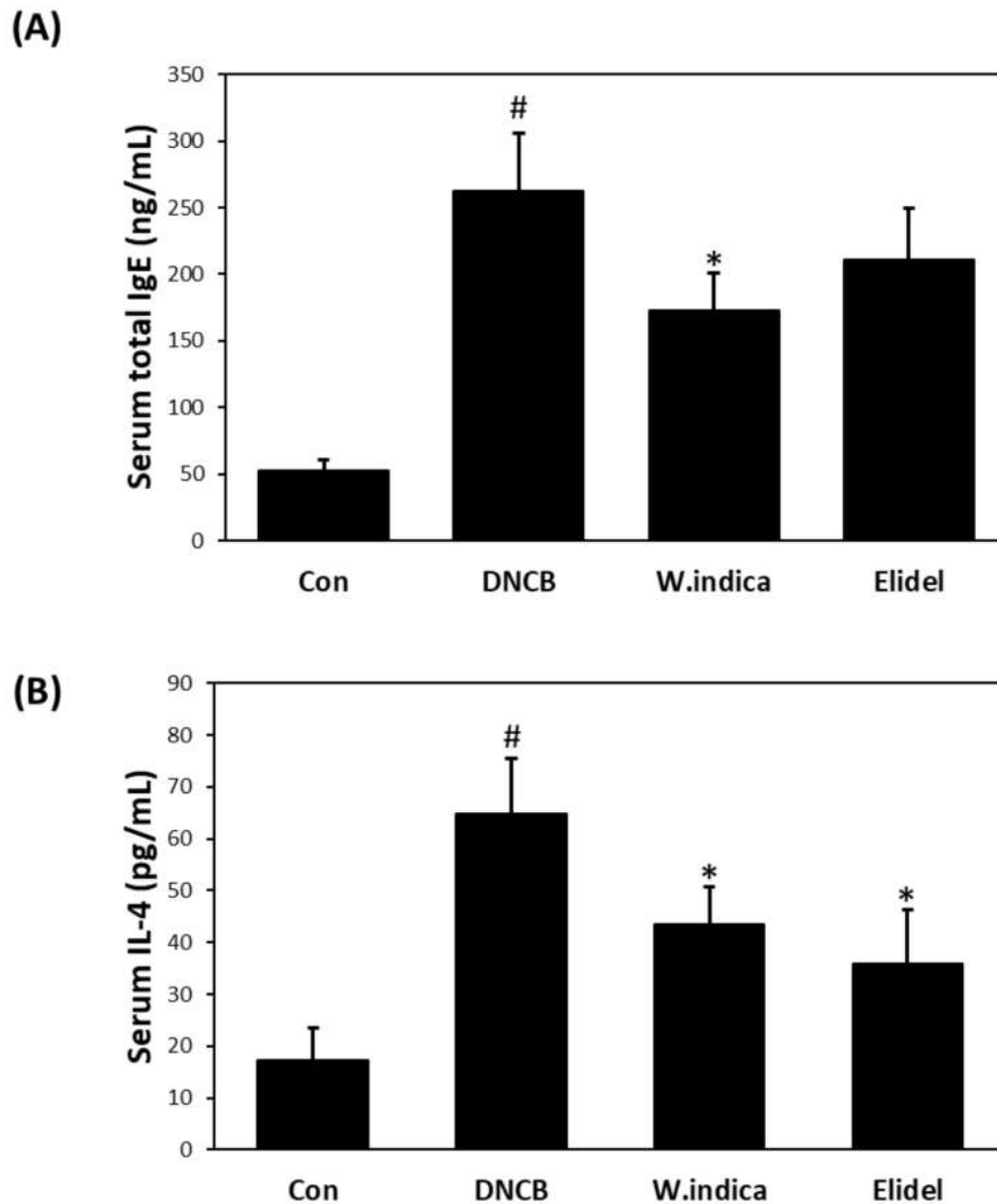
Figure 4. Effects of W. indica on serum IgE and IL-4 levels. (A) Serum IgE levels. (B) Serum IL-4 levels. Results are expressed as the means \pm SEMs ( n = 7 ) of two independent experiments. # p < 0.05 vs. the CON group; * p < 0.05 vs. the DNCB group. CON: vehicle control group; DNCB: DNCB + vehicle treated group; DNCB + W. indica : DNCB and 1% W. indica extract treated group; and DNCB + Elidel: DNCB and 1% pimecrolimus treated group.
