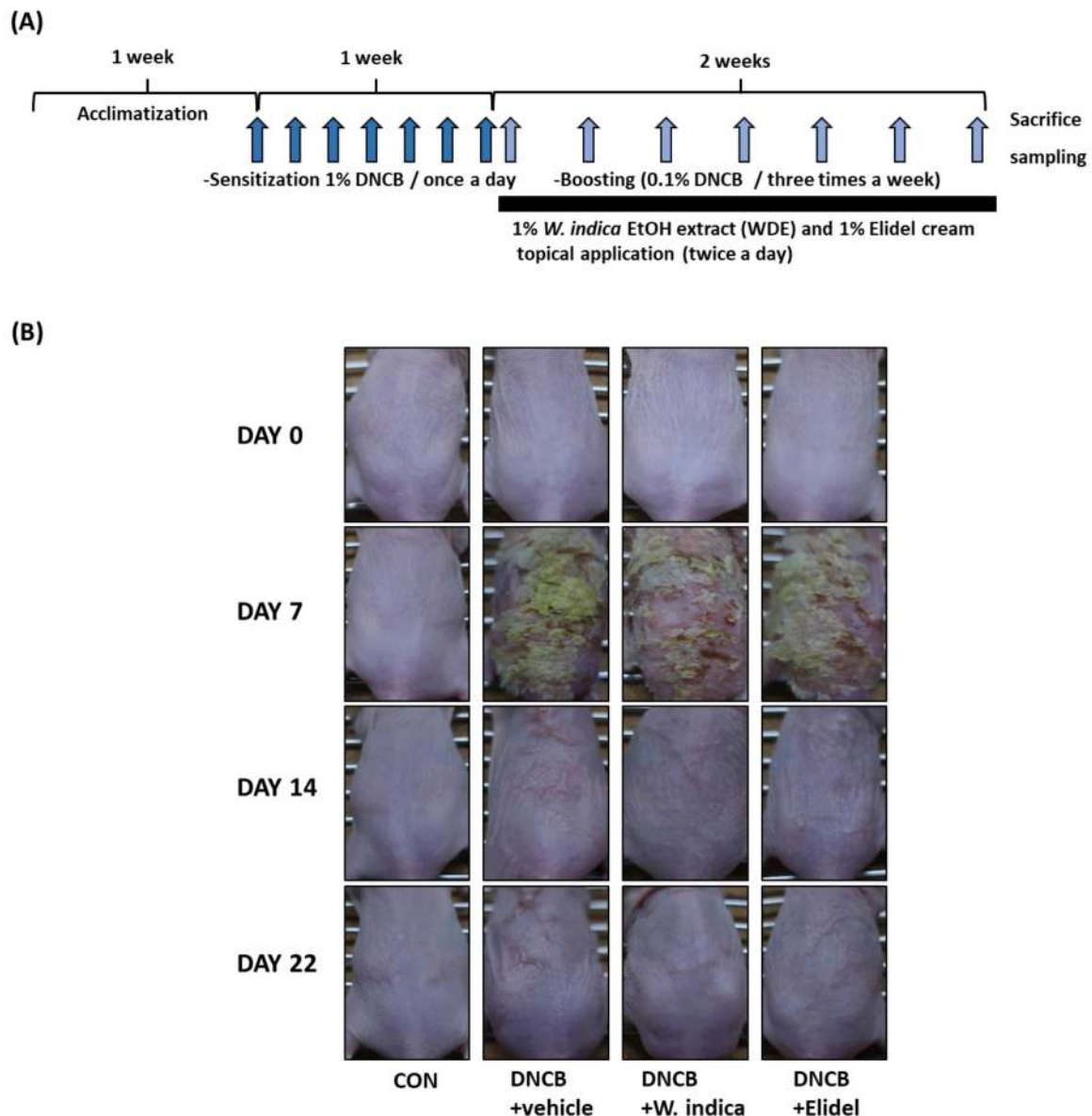
Figure 1. Effects of W. indica on the development of 2,4-dinitrochlorobenzene (DNCB)-induced AD-like skin lesions in SKH-1 hairless mice. (A) Schematic representation of the experiment. (B) Clinical features of DNCB-induced AD-like skin symptoms. CON: vehicle control group; DNCB + vehicle: DNCB-treated control group; DNCB + W. indica : DNCB plus 1% W. indica -extract treated group; and DNCB + Elidel: DNCB plus 1% pimecrolimus treated group.
