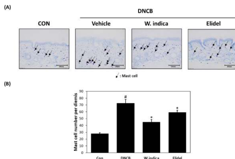
Figure 3. Effects of W. indica extract on toluidine blue staining findings and mast cell numbers in dermal tissues. (A) Toluidine blue staining result. (B) Mast cell numbers. Results are expressed as the means \pm SEMs of two independent experiments. # p < 0.05 vs. the CON group; * p < 0.05 vs. the DNCB group. CON: vehicle control group; DNCB: DNCB + vehicle treated group; DNCB + W. indica : DNCB and 1% W. indica extract treated group; and DNCB + Elidel: DNCB and 1% pimecrolimus treated group.
