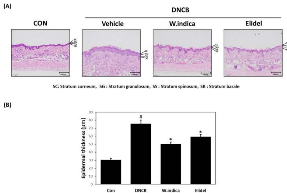
Figure 2. Effects of W. indica extract on hematoxylin and eosin (H & E) histopathology findings and epidermal thickness. (A) H & E staining result. (B) Epidermal thickness. Results are expressed as the means \pm SEMs of two independent experiments. # p < 0.05 vs. the CON group; * p < 0.05 vs. the DNCB group. CON: vehicle control group; DNCB: DNCB + vehicle treated group; DNCB + W. indica : DNCB and 1% W. indica extract treated group; and DNCB + Elidel: DNCB and 1% pimecrolimus treated group.
