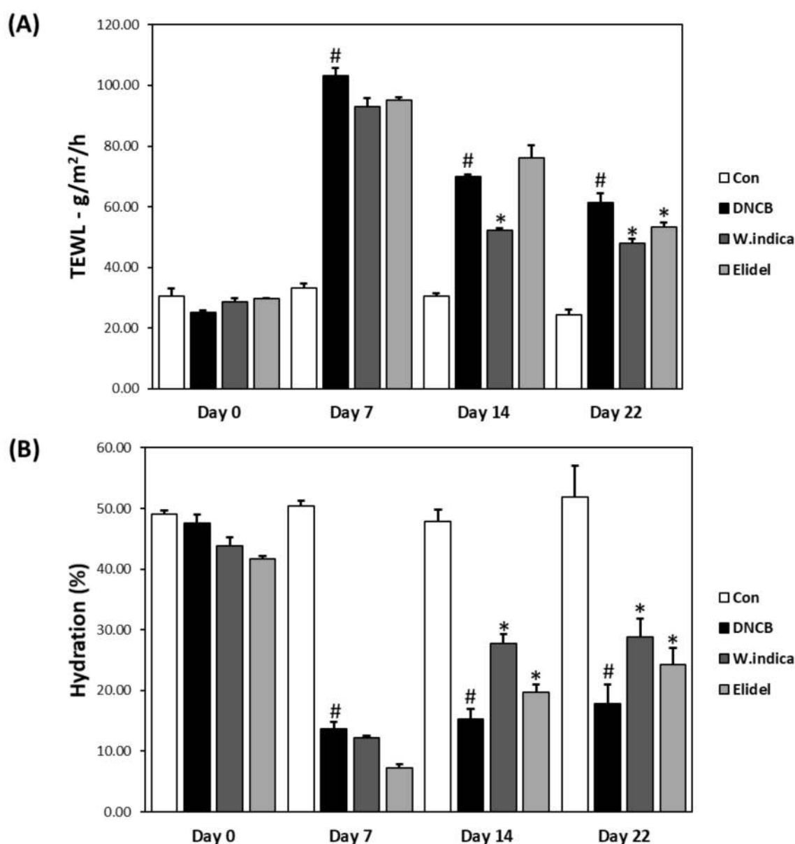
Figure 5. Effects of W. indica extract on skin barrier function. (A) Transepidermal water loss (TEWL). (B) Skin hydration values. Results are expressed as the means \pm SEMs (n = 7) of two independent experiments. # p < 0.05 vs. the CON group; * p < 0.05 vs. the DNCB group. CON: vehicle control group; DNCB: DNCB + vehicle treated group; DNCB + W. indica : DNCB and 1% W. indica extract treated group; and DNCB + Elidel: DNCB and 1% pimecrolimus treated group.
