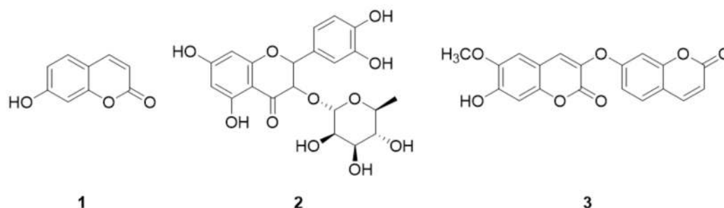
Figure 6. HPLC chromatogram of the phenolic compounds of Wikstroemia indica (A) and the chemical structures of its major compounds (B). Phytochemical characterization of the W. indica EtOH extract was performed using HPLC/MS. 1: umbelliferone ( t_R 12.368 min), 2: quercitrin ( t_R 22.718 min), and 3: daphnoretin ( t_R 27.377 min).
