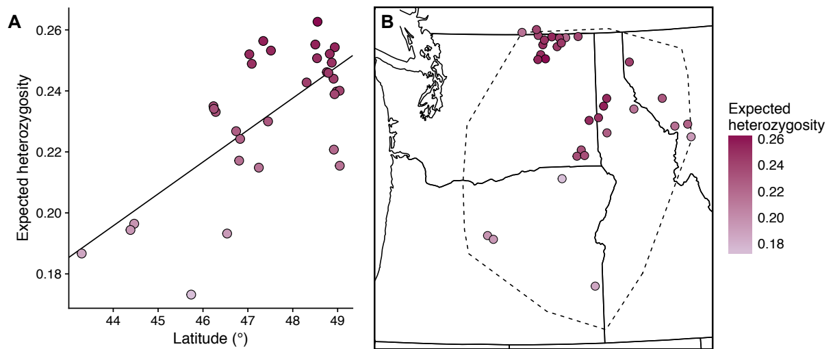
Figure 6 (A) Expected heterozygosity increases with latitude across the range of Clarkia pulchella . (B) Expected heterozygosity appears to be higher in central and northern parts of the range, but lower in the south and east.
