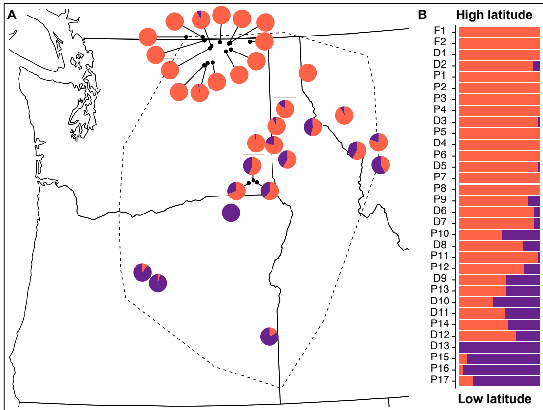
Figure 5 Admixture proportions of each of 32 populations of Clarkia pulchella estimated from by conStruct with K = 2 . A Admixture proportions are shown in geographic space and (B) arranged by latitude . Population ID codes are consistent with Table S1 and Figure 1.
