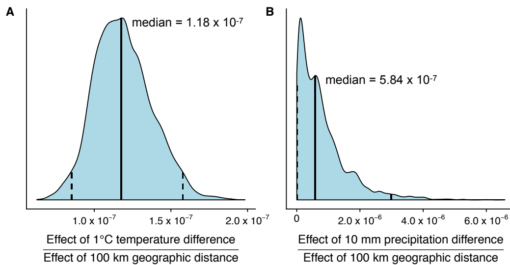
Figure S1 Marginal posterior distributions, median values (solid lines) and 95% credible intervals (dashed lines) of the ratio of the effect sizes of (A) temperature vs. geographic distance and (B) spring/summer precipitation vs. geographic distance on genetic differentiation of populations of Clarkia pulchella after a burn-in of 20%.
