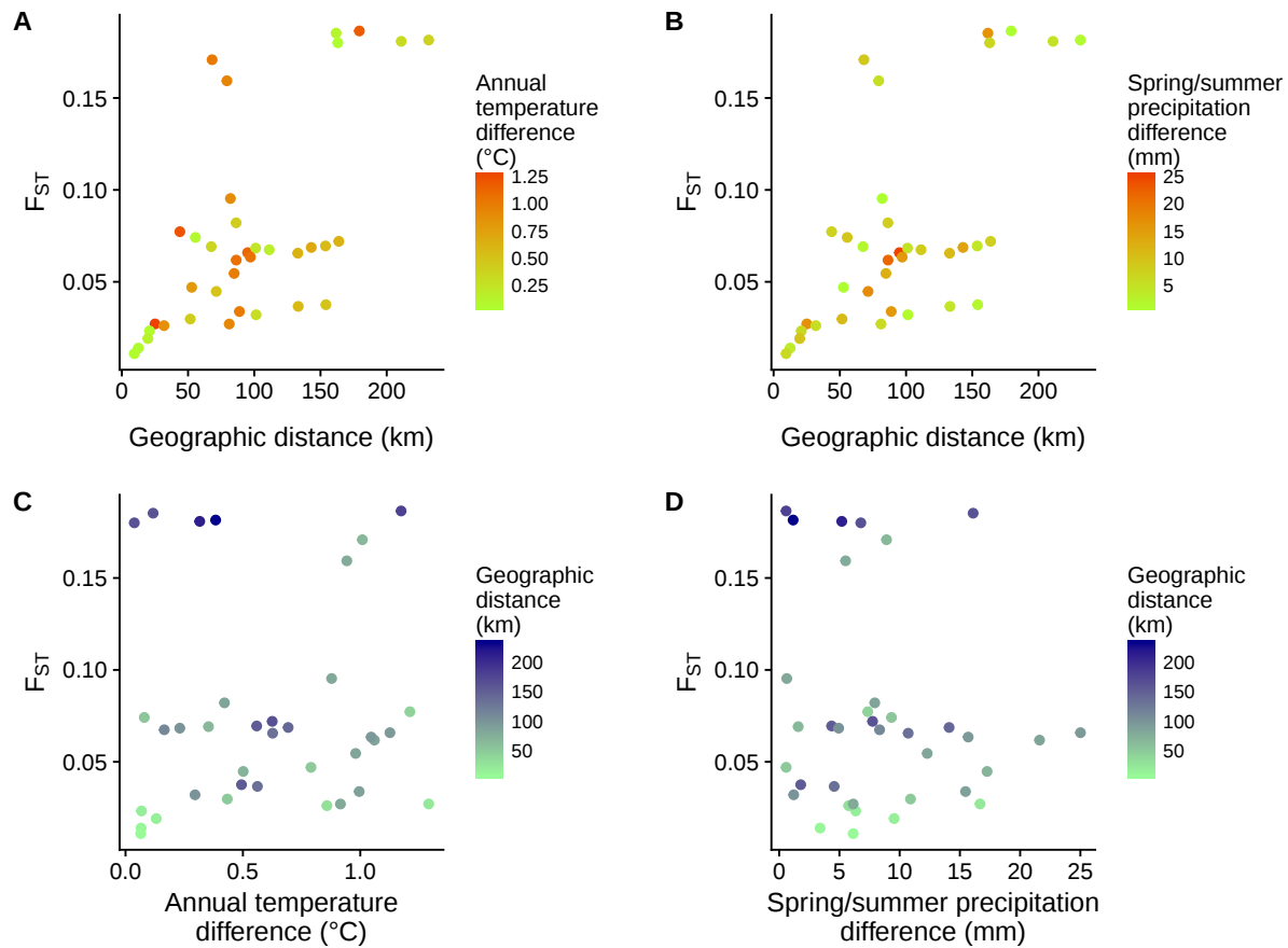
Figure S3 Relationship between pairwise geographic distance (x-axis in A and B ), temperature differences (color in A ) or precipitation differences (color in B ), and genetic differentiation ( F_{ST} ) among populations in the central part of the geographic range of Clarkia pulchella . An alternative visualization is presented in (C) and (D) , in which climate differences are plotted on the x-axis and geographic distance is indicated with color. Climate data are 1951-1980 averages from PRISM (PRISM Climate Group, 2017).
