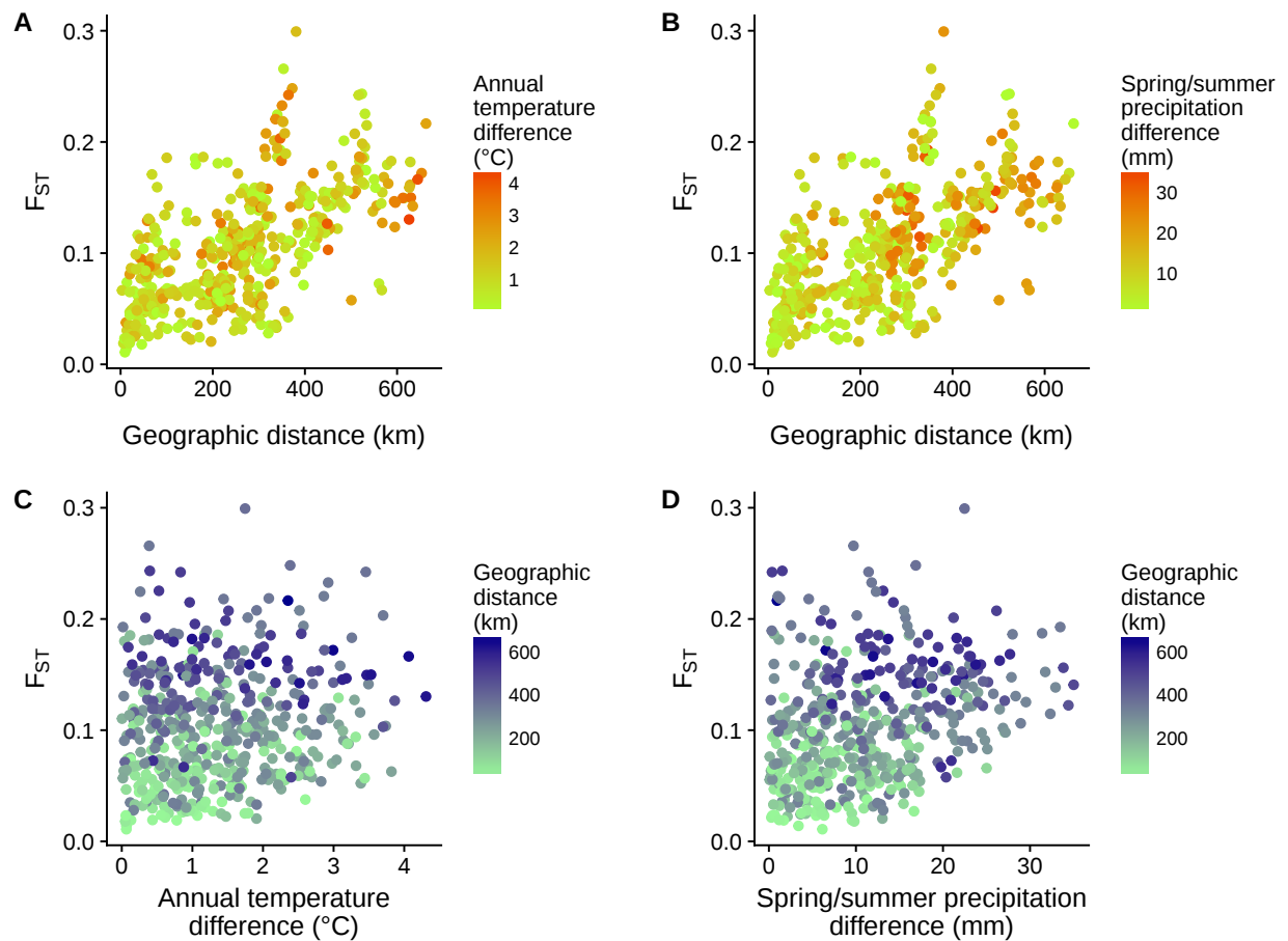
Figure 3 Pairwise genetic differentiation ( F_{ST} ) of populations of Clarkia pulchella increases with geographic distance (x-axis in A and B ), but shows no discernible relationship to temperature differences (color in A ) or precipitation differences (color in B ). An alternative visualization is presented in ( C ) and ( D ), in which climate differences are plotted on the x-axis and geographic distance is indicated with color. Climate data are 1951-1980 averages from PRISM (PRISM Climate Group, 2017).
