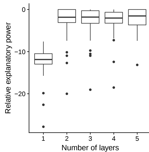
Figure 4 Results of 100 replicate cross-validation runs of conStruct with the number of layers set to 1, 2, 3, 4, or 5. In each replicate, the model is built using 90% of loci, and the log-likelihood of the remaining loci is calculated. Predictive accuracy is then calculated as the difference in log-likelihood between each model and the best model (i.e. the best number of layers) in each replicate. These results indicate that models constructed with two layers are best, because they provide as much explanatory power as other models without further complexity.
