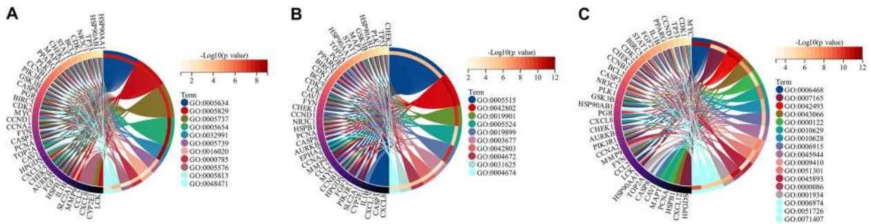
Fig. 5 GO functional enrichment of the ACP-colon key targets. A Cellular component. GO:0005634, nucleus; GO:0005829, cytosol; GO:0005737, cytoplasm; GO:0005654, nucleoplasm; GO:0032991, macromolecular complex; GO:0005739, mitochondrion; GO:0016020, membrane; GO:0000785, chromatin; GO:0005576, extracellular region; GO:0005813, centrosome; GO:0048471, perinuclear region of cytoplasm. B Molecular function. GO:0005515, protein binding; GO:0042802, identical protein binding; GO:0019901, protein kinase binding; GO:0005524, ATP binding; GO:0019899, enzyme binding; GO:0003677, DNA binding; GO:0042803, protein homodimerization activity; GO:0004672, protein kinase activity; GO:0031625, ubiquitin protein ligase binding; GO:0004674, protein serine/threonine kinase activity. (C) Biological process. GO:0006468, protein phosphorylation; GO:0007165, signal transduction; GO:0042493, response to drug; GO:0043066, negative regulation of apoptotic process; GO:0000122, negative regulation of transcription from RNA polymerase II promoter; GO:0010629, negative regulation of gene expression; GO:0010628, positive regulation of gene expression; GO:0006915, apoptotic process; GO:0045944, positive regulation of transcription from RNA polymerase II promoter; GO:0009410, response to xenobiotic stimulus; GO:0051301, cell division; GO:0045893, positive regulation of transcription, DNA-templated; GO:0000086, G2/M transition of mitotic cell cycle; GO:0001934, positive regulation of protein phosphorylation; GO:0006974, cellular response to DNA damage stimulus; GO:0051726, regulation of cell cycle; GO:0071407, cellular response to organic cyclic compound
