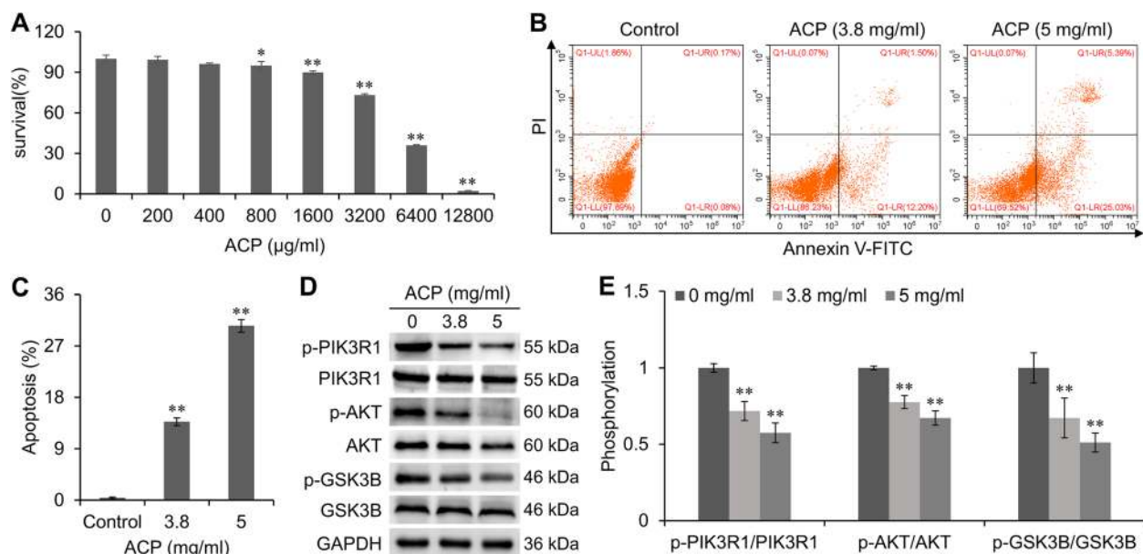
Fig. 9 Anticancer effects of ACP against CT26 cells. A Cell proliferation was detected using CCK-8 assay. B, C Apoptosis was identified by flow cytometry. D, E proteins expression and phosphorylation were evaluated by Western blot. Compared with control group, * P < 0.05 , ** P < 0.01
