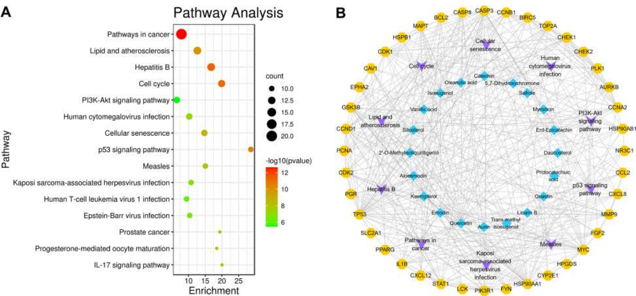
Fig. 6 Pathway enrichment of the ACP-colon key targets. A KEGG pathway enrichment analysis. B Compound–key target–pathway network. Blue diamond nodes represent the compounds in ACP. Violet V nodes represent the pathway. Orange octagon nodes represent the key targets of ACP
