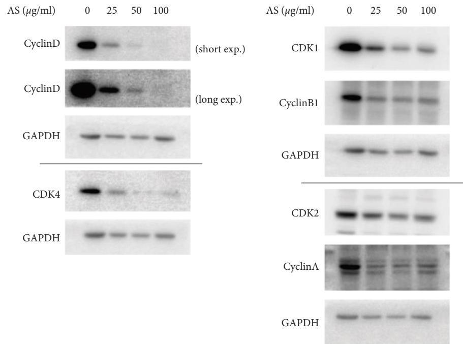
FIGURE 2: AS reduces the protein levels of CDK1, CDK2, and CDK4 and Cyclin B1, Cyclin A, and Cyclin D in LNCaP cells. LNCaP cells were seeded in 12-well plates and then treated with AS extracts (0, 25, 50, and 100 \mu\text{g/ml} ) for 24 hours. Western blot analysis was performed to evaluate the protein expression of cell cycle regulators with specific primary antibodies targeting CDK1, CDK2, CDK4, Cyclin A, Cyclin B1, and Cyclin D. GAPDH was served as an internal control.
