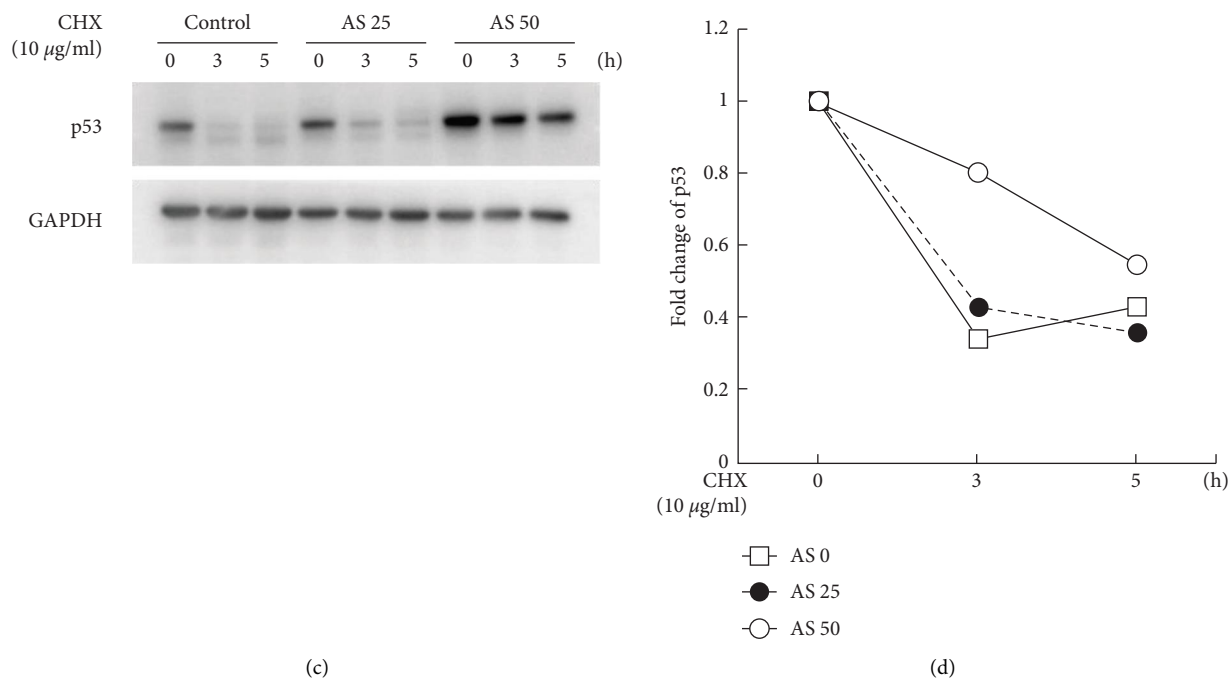
FIGURE 3: AS increases the protein level of p53 and reduces its protein degradation. (a) LNCaP cells were seeded in 12-well plates and followed with the treatment of AS with a series of concentrations (0, 6.25, 12.5, 25, 50, and 100 µg/ml) for 24 hours. Western blot analysis was performed to identify the protein levels of p53 after AS treatment, and the protein level of GAPDH was served as an internal control. (b) The quantitative results of (a) were shown. (c) LNCaP cells were seeded in 12-well plates and then treated with AS (0, 25, and 50 µg/ml) for 24 hours. After that, the cells were treated with 10 µg/ml cycloheximide for 0, 3, and 5 hours before protein extraction. Western blot analysis was then performed to evaluate the protein level of p53 with specific p53 antibody. (d) The quantitative data of the p53 degradation curves were shown and the original p53 protein levels of all groups were adjusted as 1. Data were presented as the mean \pm S.E.M. (Standard error of the mean) with three independent experiments ( n=3 ) and the paired Student's t -test was used to calculate the p -value compared to group = 0. Significance was marked as * p < 0.05 , ** p < 0.01 , and *** p < 0.001 .
