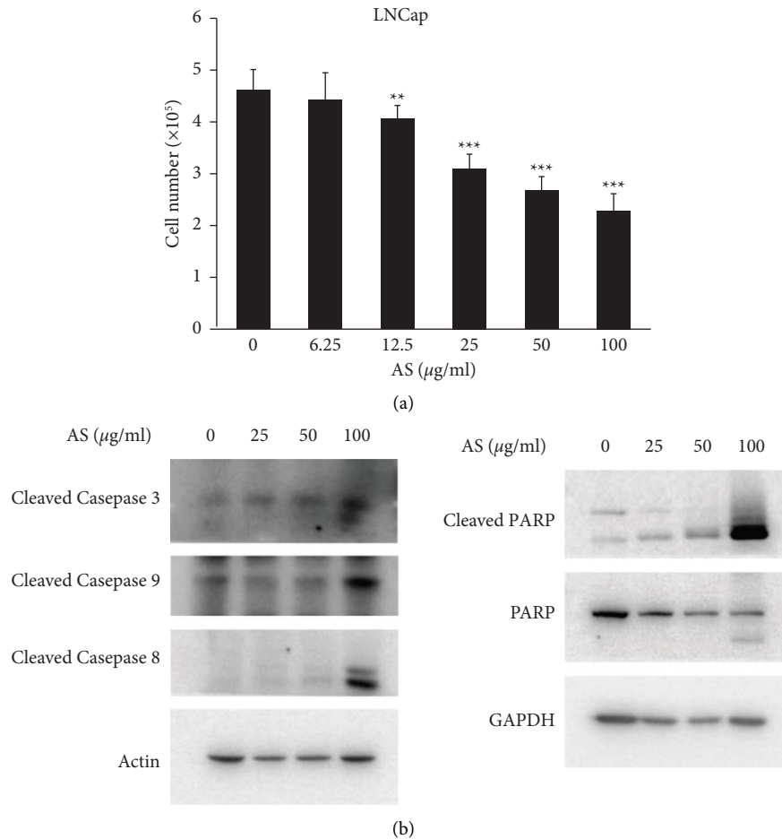
FIGURE 1: AS induces apoptosis of LNCaP cells. (a) LNCaP cells were seeded in 12-well plates and then treated with 6.25, 12.5, 25, 50, and 100 \mu\text{g/ml} AS for 24 hours followed by trypan blue assay. Data were presented as the mean \pm S.E.M. (Standard error of the mean) with three independent experiments ( n=3 ) and paired Student's t -test was used to calculate the p -value. Statistical significance was marked as *p < 0.05 , **p < 0.01 , and ***p < 0.001 . (b) LNCaP cells were seeded in 12 well plates and then treated with AS (0, 25, 50, and 100 \mu\text{g/ml} ) for 24 hours. Protein expression of apoptotic markers was evaluated by western blot with the specific primary antibodies anticlaved PARP, anti-PARP, anticlaved caspase 3, anticlaved caspase 8, anticlaved caspase 9, anti-GAPDH, and antiactin. GAPDH and actin were served as internal controls.
