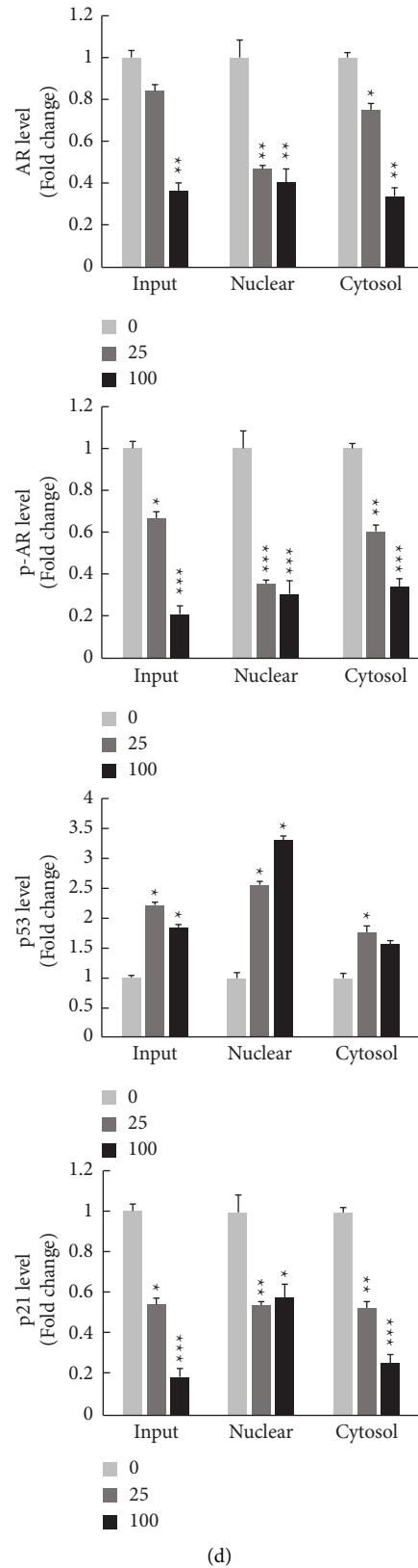
FIGURE 4: AS reduces expression and phosphorylation of AR, and causes nuclear localization of p53. (a) LNCaP cells were seeded in 12-well plates and then treated with AS (0, 6.25, 12.5, 25, 50, and 100 \mu\text{g/ml} ) for 24 hours. Western blot analysis was performed to evaluate the protein levels of AR phosphorylation at Ser-81 and total AR in LNCaP cells. (b) The quantitative results of (a) were shown, where actin was used as an internal control. (c) LNCaP cells were treated with AS (0, 25, and 100 \mu\text{g/ml} ) for 24 hours. Protein extraction was performed by nucleus/cytosol cell fractionation. Protein levels were detected by western blotting with specific antibodies targeting AR, p-s81-AR, p53, p21, and PARP. Actin protein was served as an internal control. PARP and tubulin were respectively served as nuclear and cytosolic markers. (d) The quantitative results of (c) were shown. Data were presented as the mean \pm S.E.M. (standard error of the mean) with three independent experiments ( n = 3 ) and the paired Student's t -test was used to calculate the p -value compared to group = 0. Significance was marked as * p < 0.05 , ** p < 0.01 , and *** p < 0.001 .
