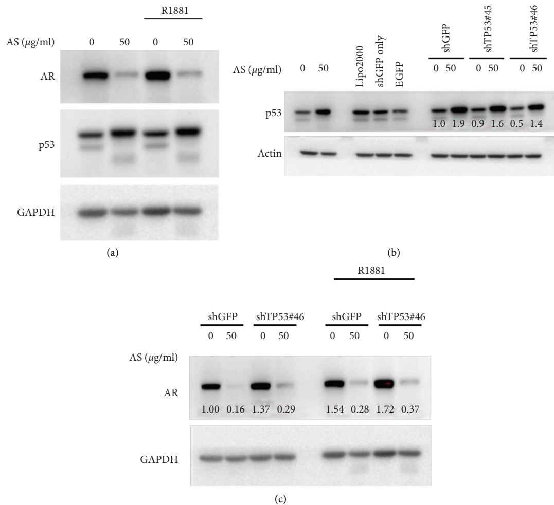
FIGURE 5: AS inhibits AR through p53 upregulation. (a) LNCaP cells were seeded in 12-well plates and then treated with AS (0, 50 \mu\text{g/ml} ) and 0.1 nM R1881 for 24 hours. (b) The expression of p53 was evaluated following knockdown of p53 by shRNA. (c) Knockdown of p53 was performed by shTP53 in LNCaP cells in the presence of R1881 (a synthetic androgen; 0.1 nM for 24 hours). The control groups were transfected with shGFP. Protein levels were detected by western blotting analysis with specific AR and p53 antibodies. GAPDH served as internal controls.
