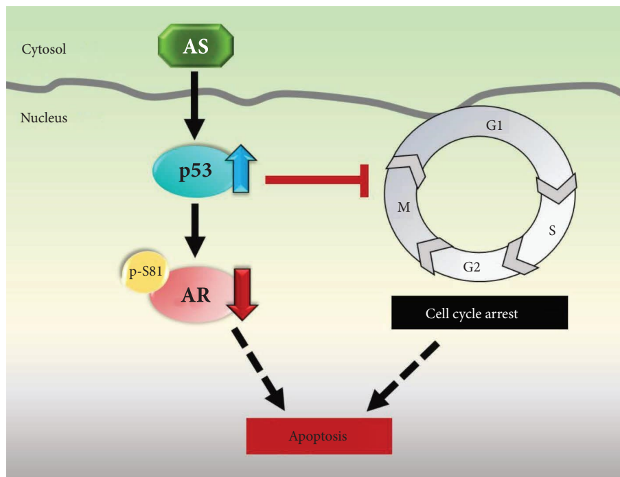
FIGURE 6: Schematic diagram of AS-mediated regulation of apoptosis in prostate cancer. AS enhances p53 protein stability and nuclear accumulation in androgen-dependent human prostate cancer cells. Increased p53 inhibits both the Ser-81 phosphorylation and protein stability of AR in the nucleus. Decreased protein expression/activation of AR through p53 upregulation, therefore, causes apoptotic features in prostate cancer cells. Besides, AS-mediated p53 activation results in cell cycle inhibition. Overall, AS inhibits prostate cancer cell proliferation through p53 regulation and AR inhibition.
